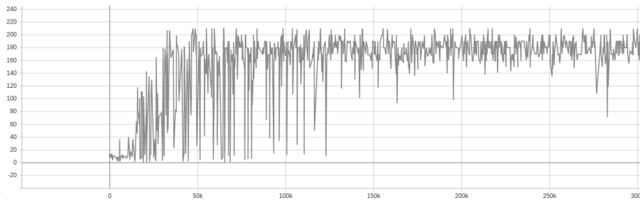
Figure 25: GridEnv, 4D, n = 20 . After around 130k iterations the model is trained. In comparison to the same configuration trained in 3D, Figure 24, the variance is slightly higher. The average reward is also a little bit lower which is expected.
