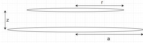
Figure 2.2: Basic two filamentary loops system
