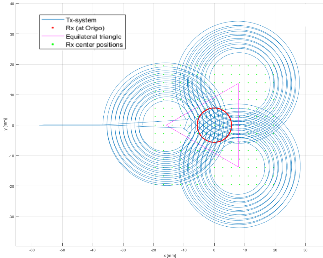
Figure 3.1: System of large Tx coils and a small Rx loop as viewed from above
