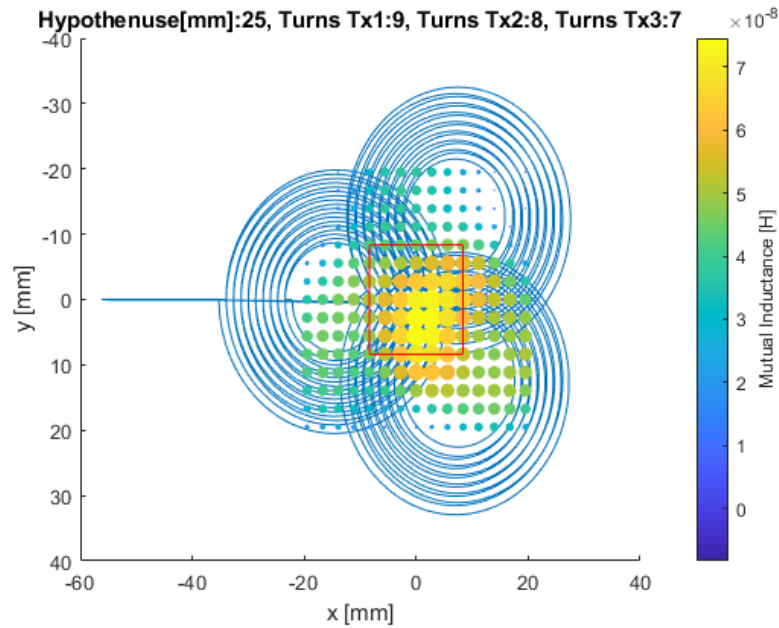
Figure 4.2: Map of mutual inductance for small receiver coil from setup 1. Initial setup with 9,8,7, Tx coil turns. Hypotenuse: 25mm
