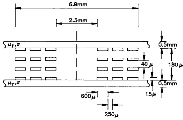
Figure 3.5: Sketch over the setup from the paper [9]
