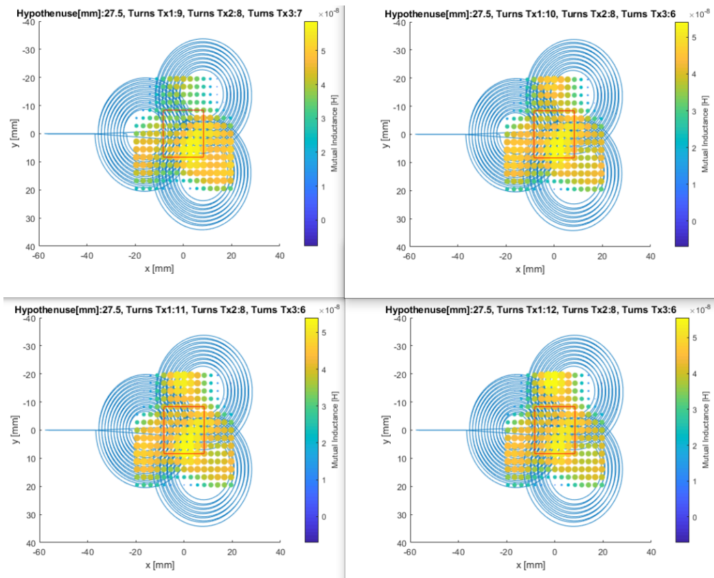
Figure 4.4: Map of mutual inductance for different Tx coil turn combinations. Hypotenuse = 27.5mm
