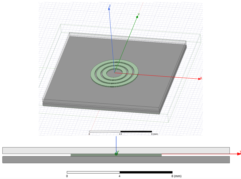
Figure 3.6: The coil setup in Ansys Maxwell
