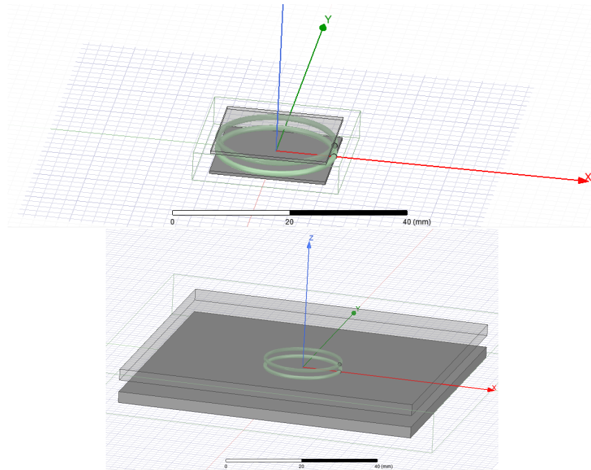
Figure 3.4: Smallest/thinnest vs. largest/thickest ferrite plates
