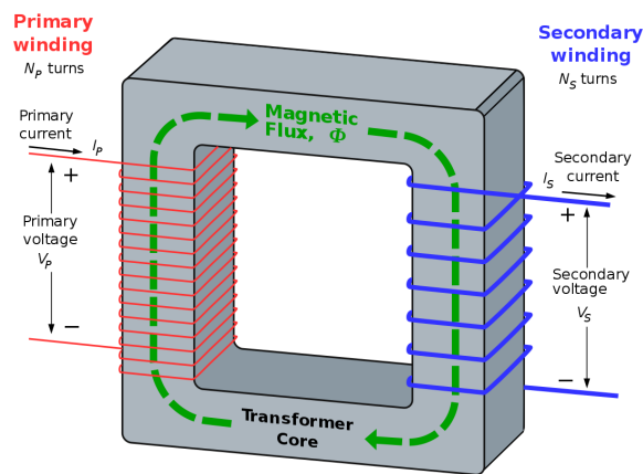
Figure 1.2: Magnetic field lines in a traditional ferrite-core transformer. Source: [4]
