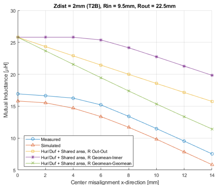
Figure 4.10: Mutual inductance for misaligned coils, z=2\text{mm} (T2B)
