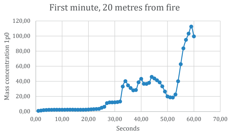
Diagram 3.5 - Mass concentration 20 meters from fire during the first minute
