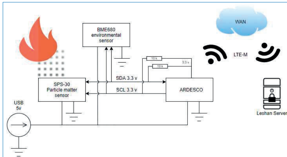
Figure 5.1 - Block diagram developed product
