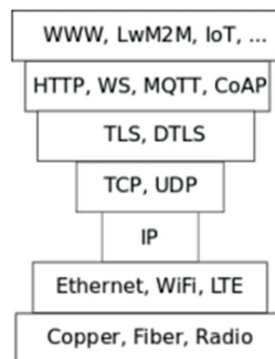
Figure 2.7 - Stack which LwM2M is built on [65]
