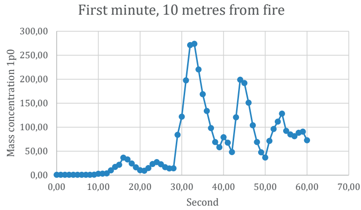
Diagram 5.4 - Mass concentration 10 meters from fire during the first minute
