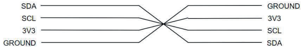
Figure 4.3 - Solution, cable spliced in a mirrored direction
