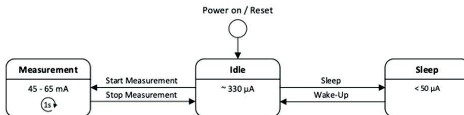
Figure 2.4 - Operating modes SPS30 [53]
