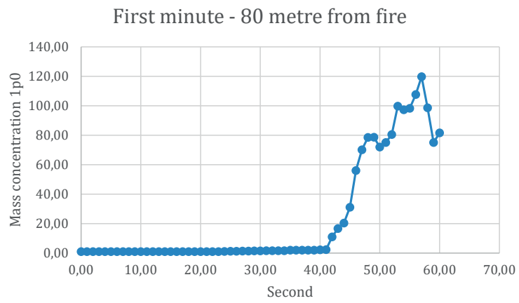
Diagram 5.4 - Mass concentration 80 meters from fire during the first minute
