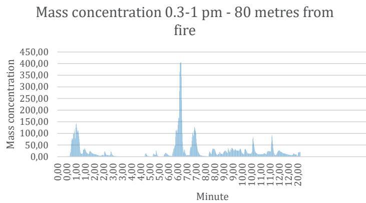
Diagram 5.3 - Mass concentration 80 meters from fire
