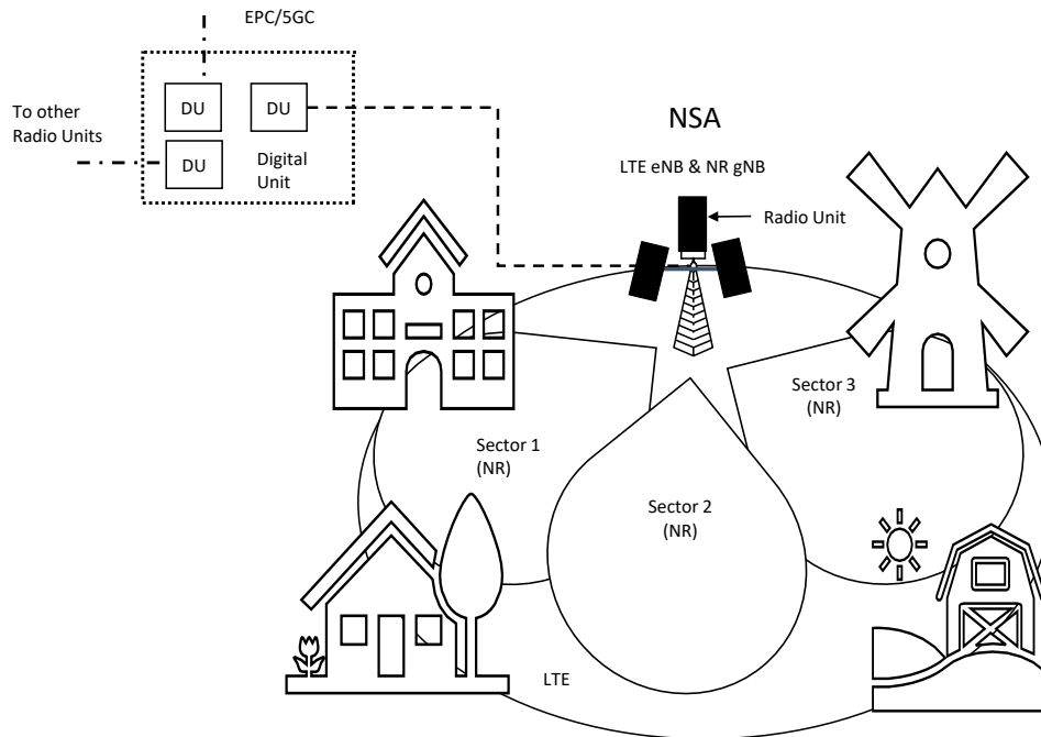
Figure 2.2: NR NSA network
