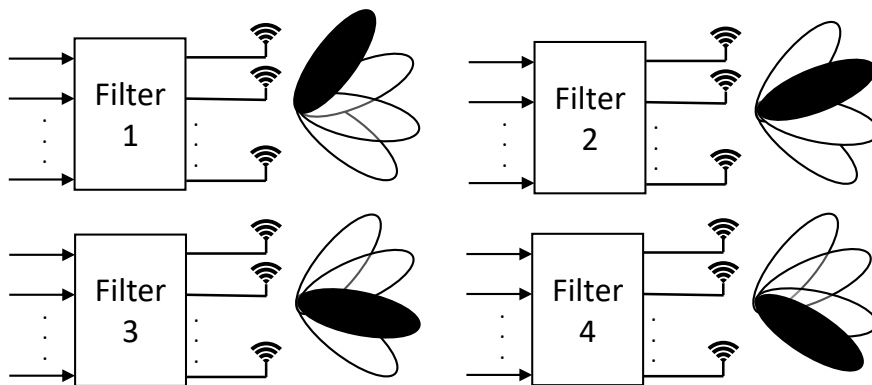
Figure 2.5: Antenna-port structure in NR
