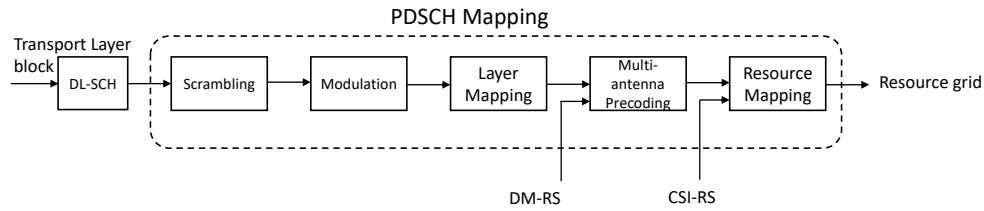
Figure 2.11: PDSCH mapping
