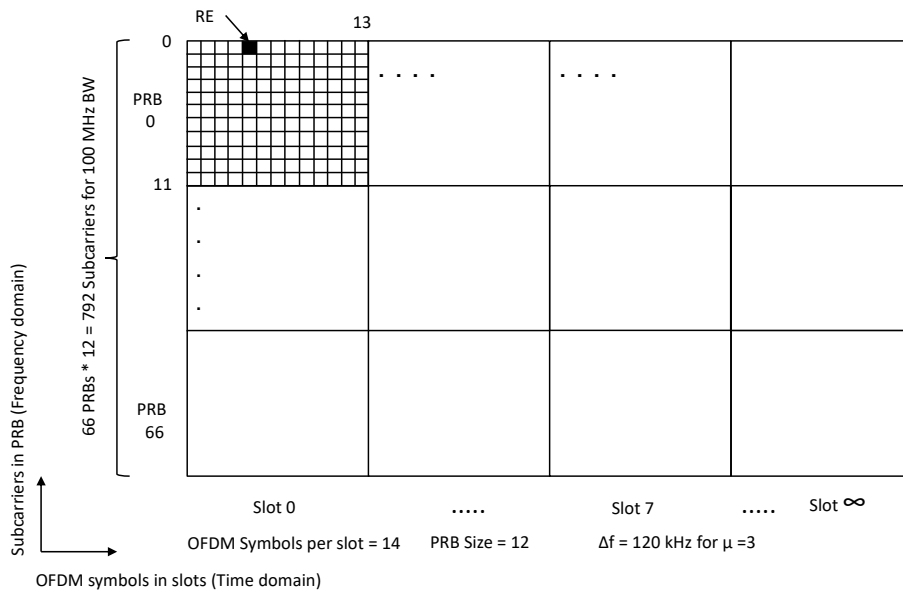
Figure 2.3: NR Time-Frequency architecture for 100 MHz bandwidth and \mu = 3
