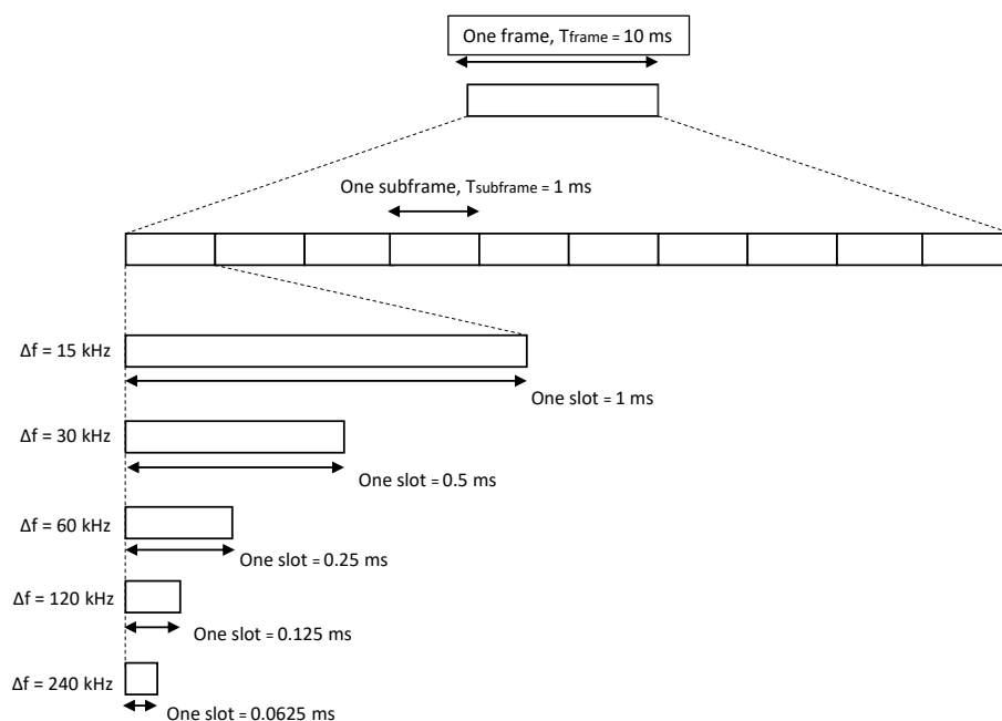
Figure 2.4: Time domain architecture in NR
