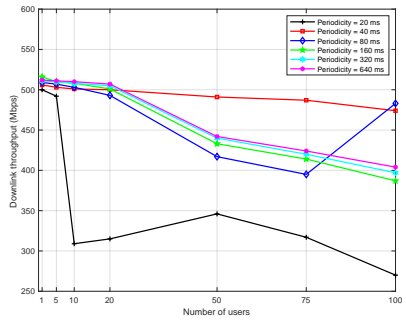
FTP DL throughput (0 km/hr)
