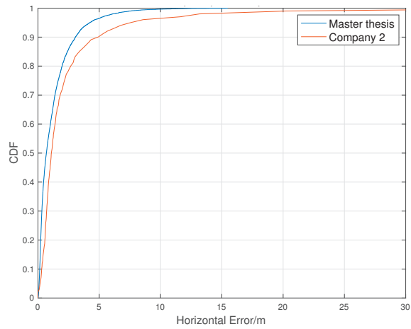
Figure 5.2: Results comparison with Company 2 in indoor office (100 MHz Bandwidth).
