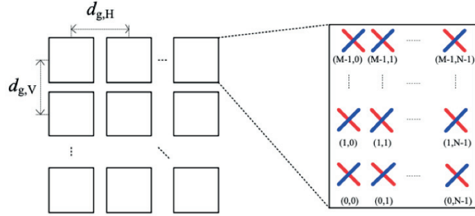
Figure 4.2: Cross-polarized panel array antenna model [10].
