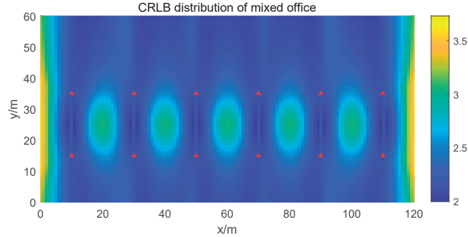
Figure 7.2: Theoretical CRLB distribution in Mixed office environment, \sigma_{\text{TOA}} * c = 3.3 m. The colour bar is in the unit meter.
