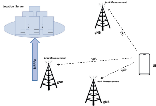
Figure 3.3: Structure of NR UL-AoA positioning.
