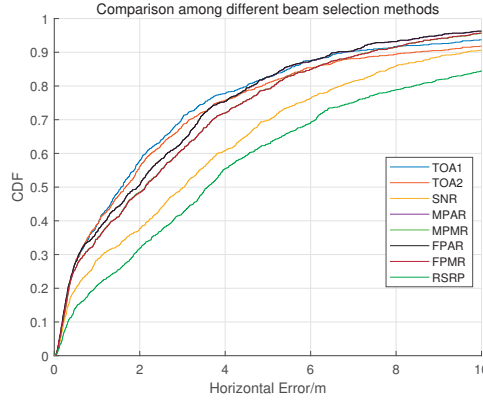
Figure 8.4: Comparison among 8 different ways of beam selection.
