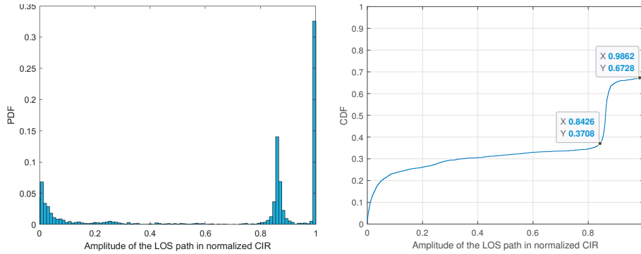
Figure 8.5: The probability density distribution and the cumulative distribution of the amplitude of the LOS path in the normalized measured CIR, simulating 3000 UEs.
