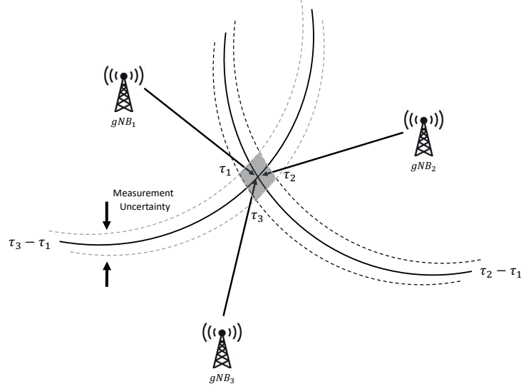
Figure 3.5: Multilateration in NR OTDOA Positioning.
