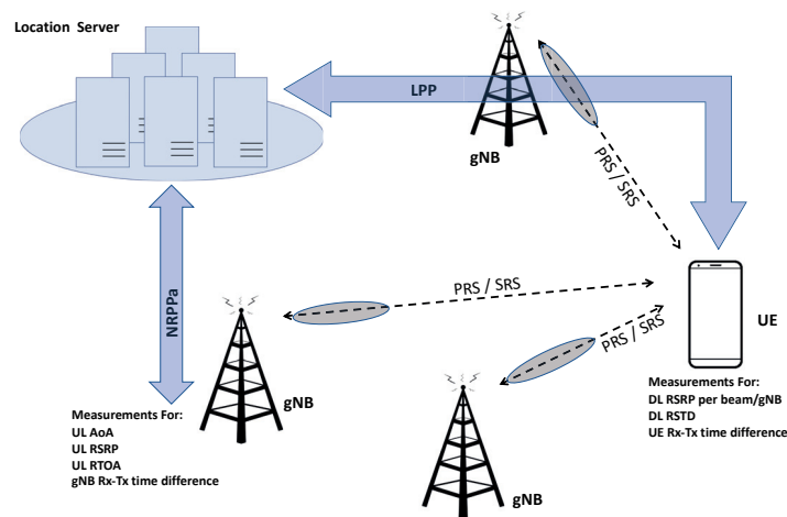
Figure 3.1: NR RAT-based positioning schemes.
