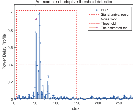
Figure 6.2: An example of adaptive threshold-based first peak detection, \beta = 0.4 , \alpha = 1 .
