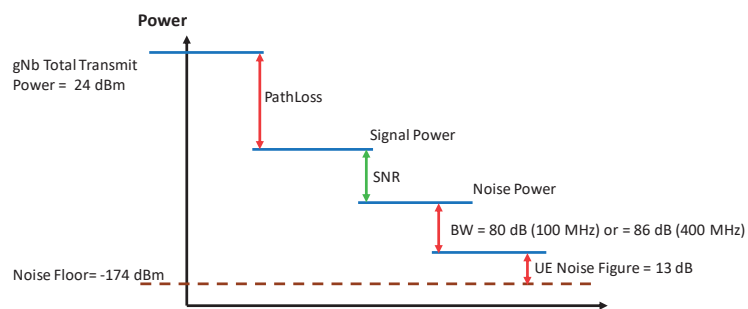
Figure 4.6: Link Budget.
