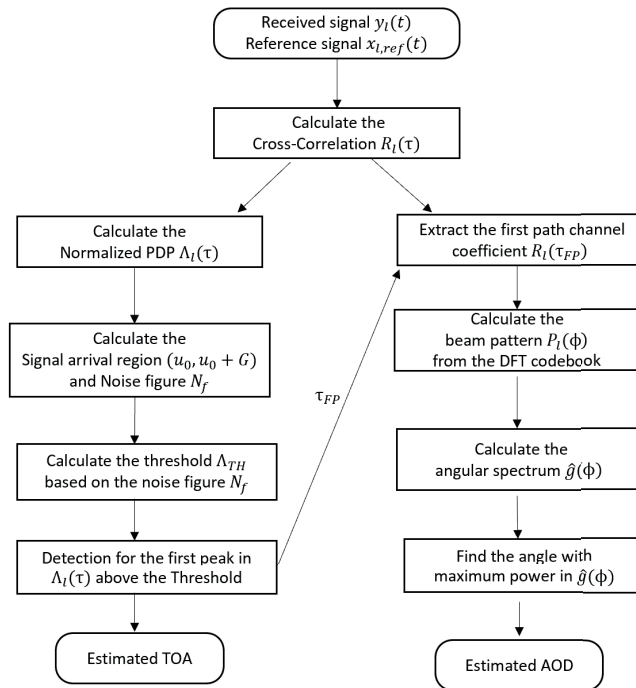
Figure 6.1: Flow chart of the TOA estimation and AoD estimation.
