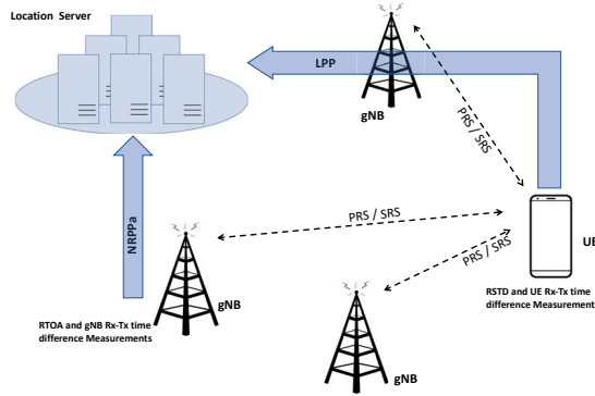
Figure 3.4: Structure of NR Multi-RTT positioning.
