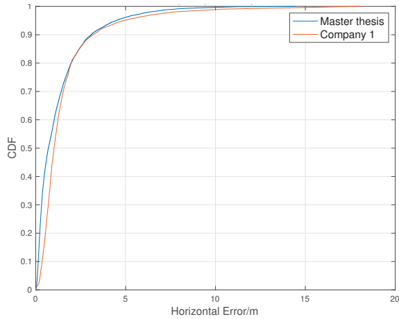
Figure 5.1: Result comparison between thesis developed simulator and Company 1 in indoor office.
