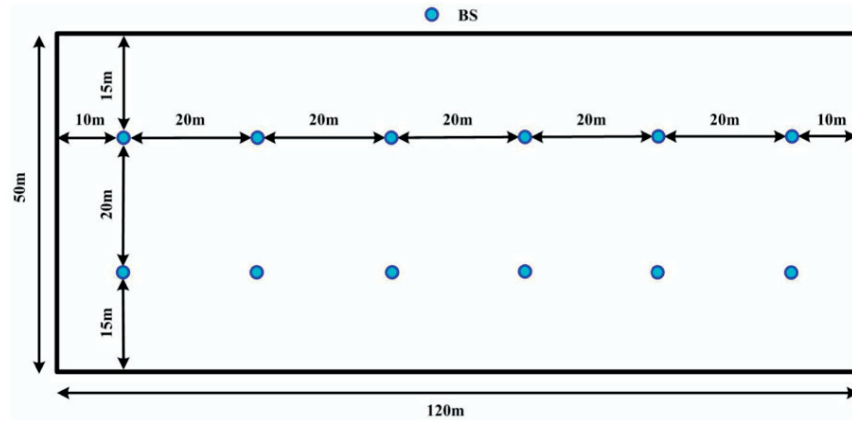
Figure 4.1: Layout of indoor office [10].
