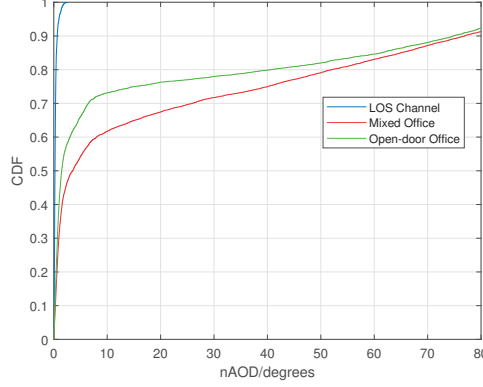
Figure 8.3: The CDF of the Angle of departure noise in Mixed office and Open office environment.
