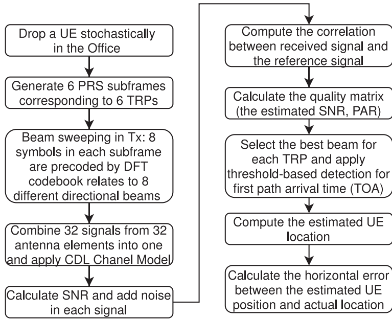
Figure 4.4: Simulation Procedure.
