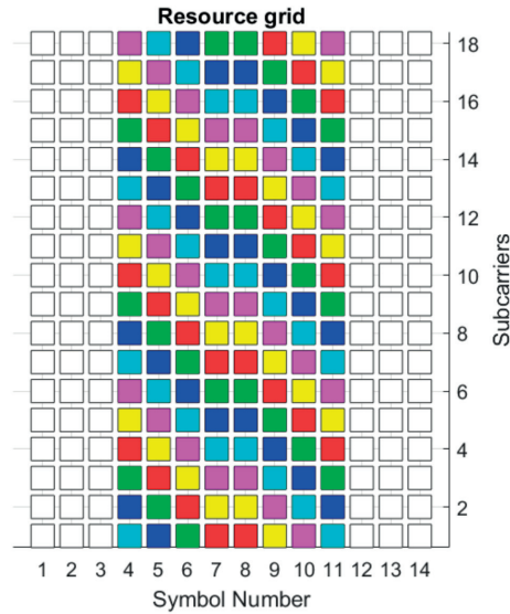
Figure 4.5: Simulation Resource Grid.
