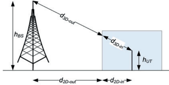
Figure 4.3: Definition of d_{2\text{D-in}} for indoor area [10].
