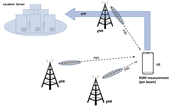
Figure 3.2: Structure of NR DL-AoD positioning.
