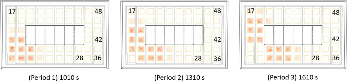
Figure 19 Fire locations in FDS during the averaging periods: (1) 1010 s, (2) 1310 s and (3) 1610 s.
