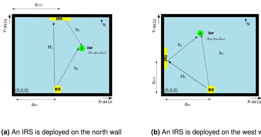
Figure 5.1: Two vertical views of the empty-room scenario geometric setup.
