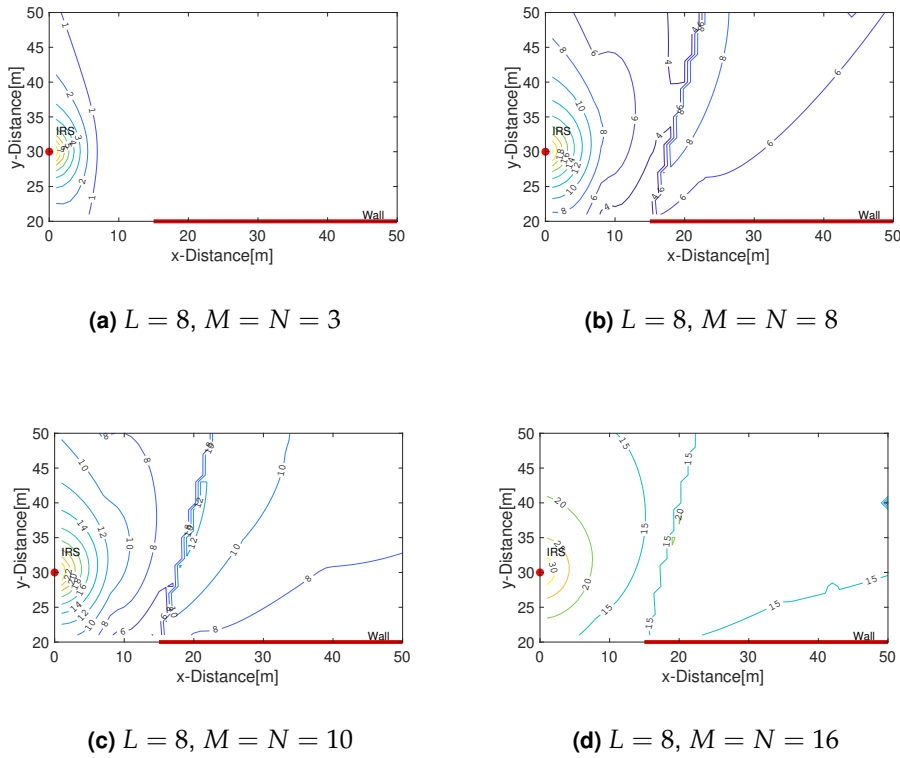
Figure 5.7: Contour plot of system power gain in dB for the geometric setup in Figure 5.6 with 7dB attenuation loss and different IRS sizes.
