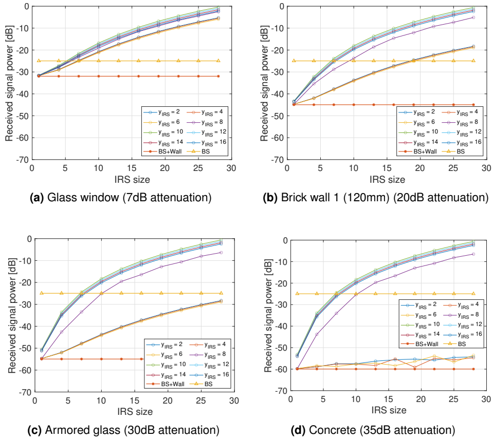
Figure 5.9: Relationship between size of IRS (side length M ) and received signal power for four different wall loss attenuation and different IRS deployment positions from y_{irs} = 2 to y_{irs} = 16 on the west wall when L = 8 .
