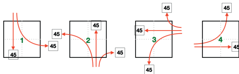
Figure A2.19. Signal phases at intersection S11 for scenario 50_150.
