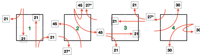
Figure A2.17. Signal phases at intersection S6 for scenario 50_150.
