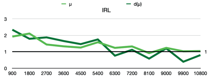
Figure 4.3. System evacuation and standard deviations of IRL.
