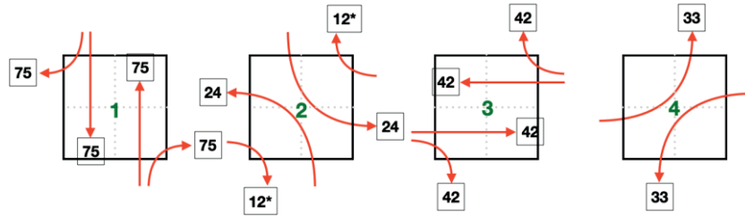
Figure A2.6. Signal phases at intersection S9 for scenario IRL.
