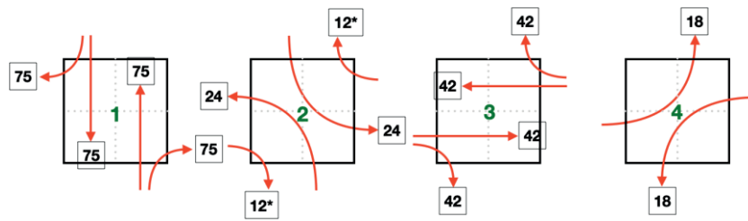
Figure A2.18. Signal phases at intersection S9 for scenario 50_150.
