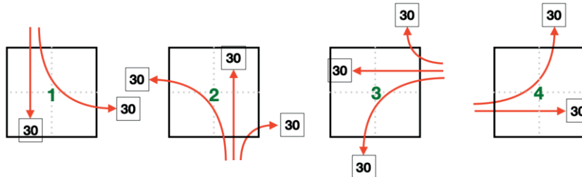
Figure A2.13. Signal phases at intersection S11 for scenario 100_33.
