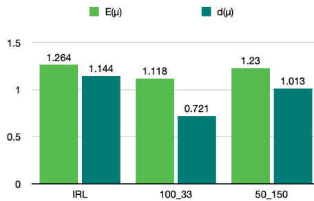
Figure 4.6. Average vehicle evacuation during t = 75 - 135 min.
