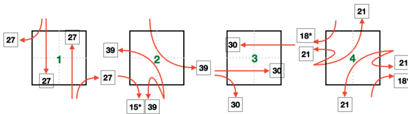
Figure A2.15. Signal phases at intersection S3 for scenario 50_150.
