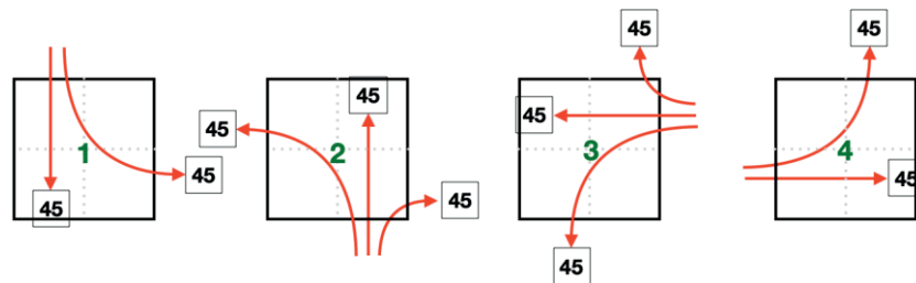
Figure A2.7. Signal phases at intersection S11 for scenario IRL.
