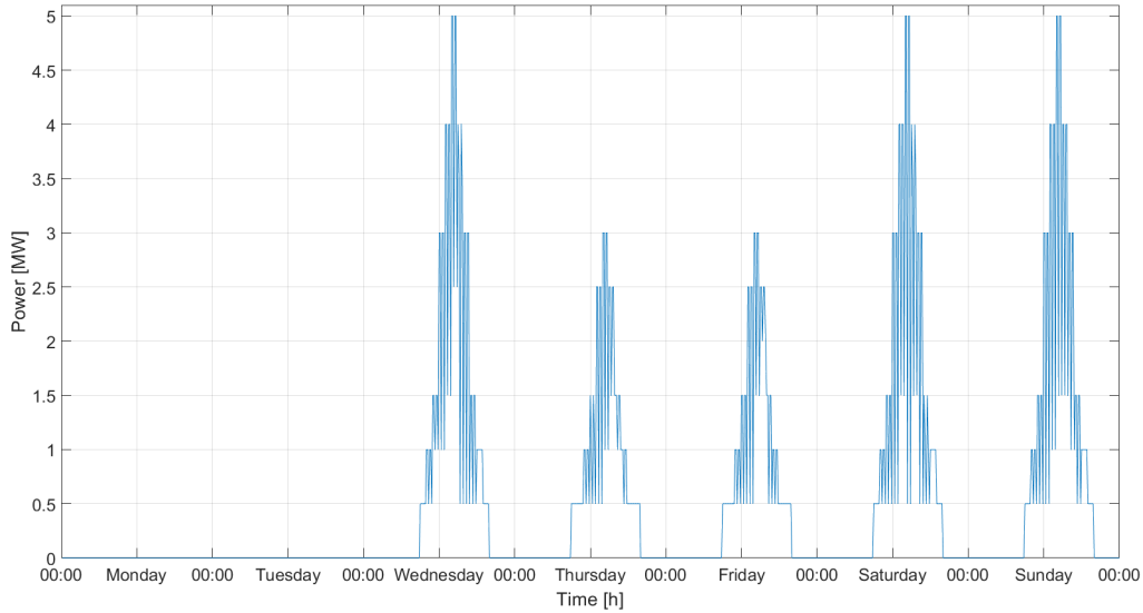
Figure 4.2: Simple charging over a week for model 2 with a maximum power demand of 5.0 MW.
