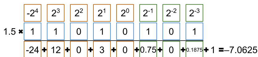
Figure 4.2: Fixed point with slope 1.5 \cdot 2^{-3} and bias +1
