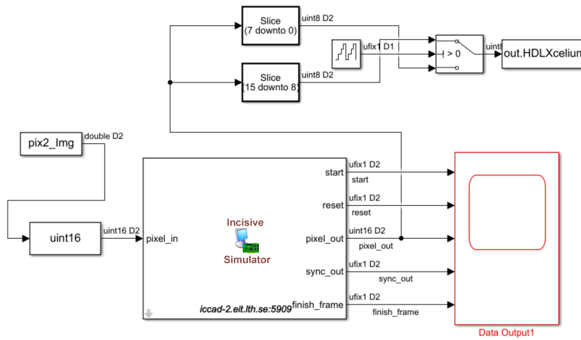
Figure 6.15: Co-simulation on Handwritten HDL
