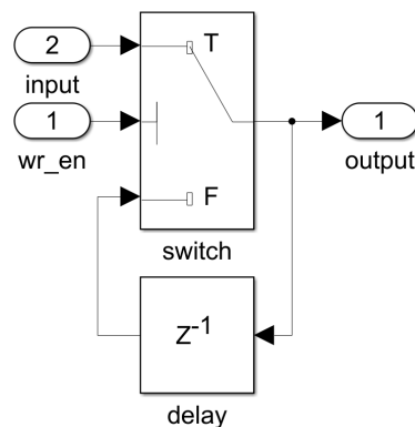
Figure 4.6: Simulink register
