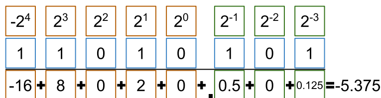
Figure 4.1: Fixed point with 3 fractional bits
