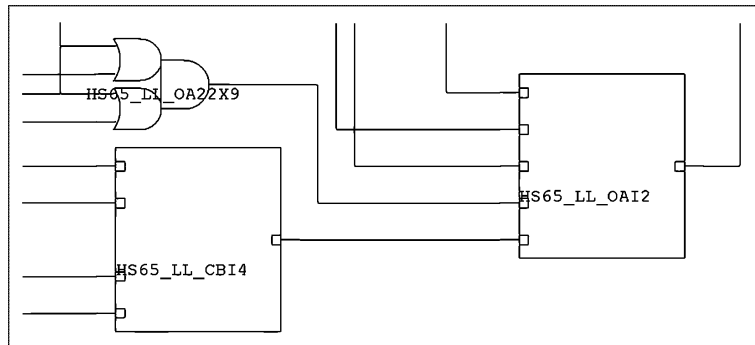
Figure 5.7: Schematic view from Genus
