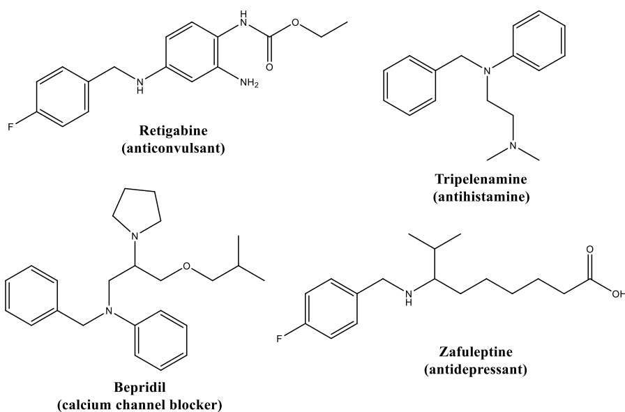
Figure 1. Various drug molecules with C-N bonds which could be synthesized by various methods.
