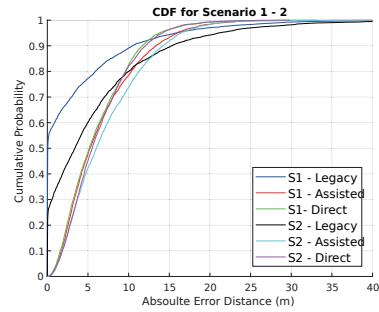
(b) CDFs for Scenario 1 and 2
