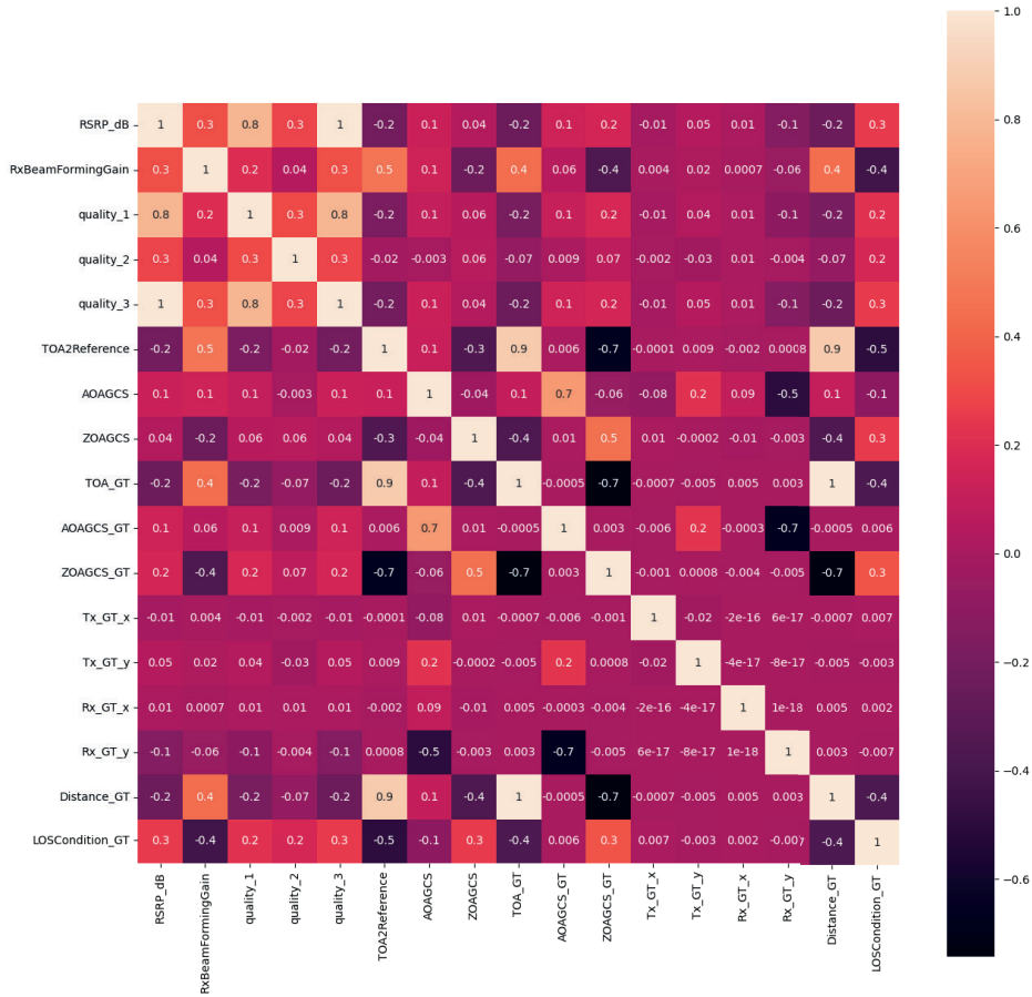
Figure 5.6: Correlation matrix for the different features
