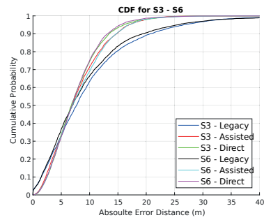
(f) CDFs for Scenario 3 and 6
