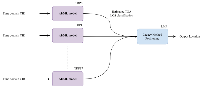
Figure 3.6: Assisted Positioning Scheme
