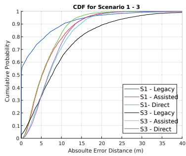
(c) CDFs for Scenario 1 and 3
