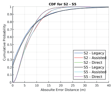
(e) CDFs for Scenario 2 and 5
