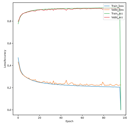
(a) SL I Complex - Training Curve for LOS prediction
