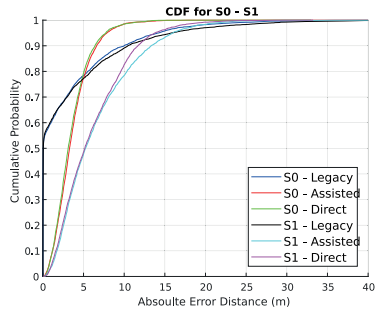
(a) CDFs for Scenario 0 and 1
