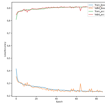
(b) SL I Simple - Training Curve for LOS prediction
