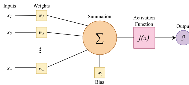
Figure 4.2: Schematics of the neuron parts
