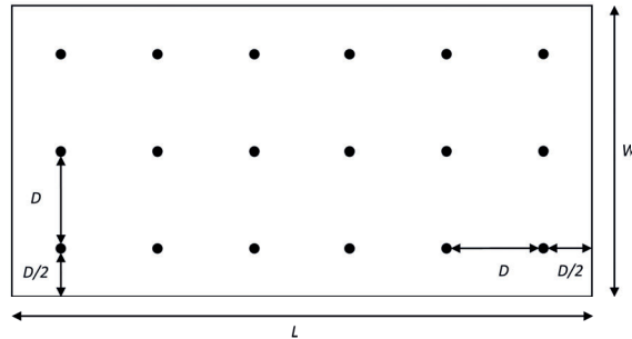
Figure 5.2: Layout of the Indoor Factory Scenario
