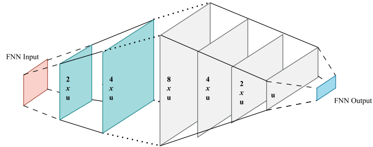
Figure 6.3: Schema of the layers structure for the single-link model with Architecture II
