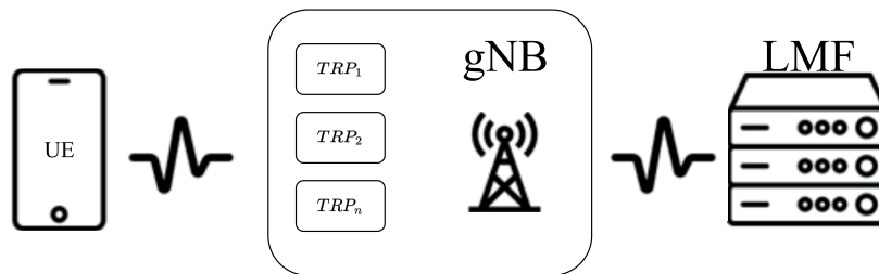
Figure 3.1: 5G Transmission and Reception Point Architecture
