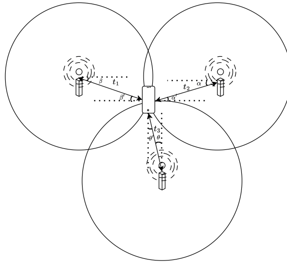
Figure 3.2: Definition of ToA/D, AoA/D
