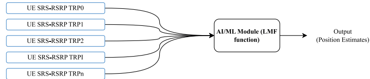
Figure 3.5: Direct Positioning Scheme
