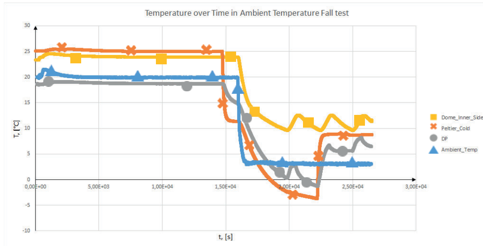
Figure 22: Data from test 4, SCC is applied.
