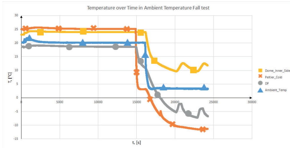
Figure 20: Data from test 3, SCC is applied.
