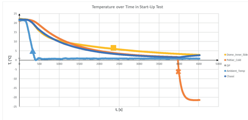
Figure 15: SCC is applied. In addition, the dark blue is the temperature of the chassis.
