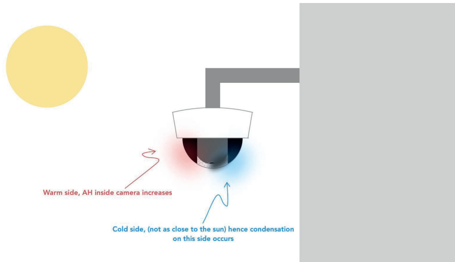
Figure 3: Demonstration of condensation during sunny/cold days.
