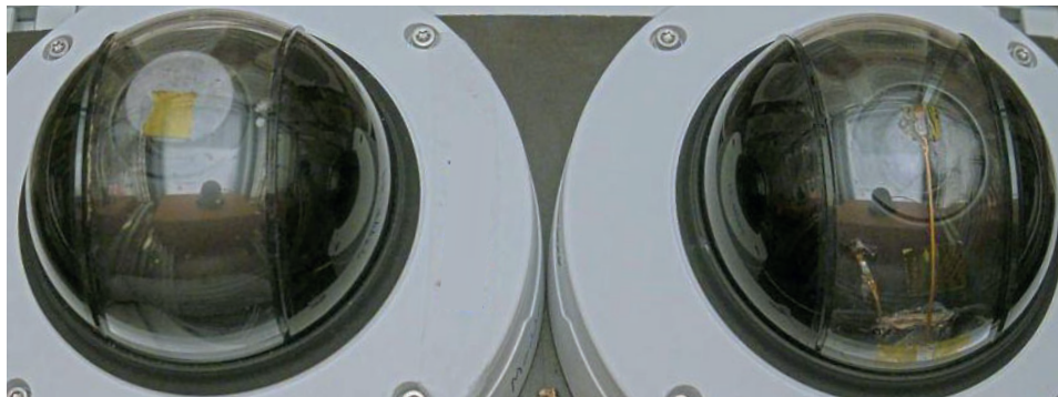
Figure 37: Image from test 6. Condensation can be seen in the left camera as a light circle in the center of the dome. A smaller, more transparent circle is visible in the center of the modified camera.
