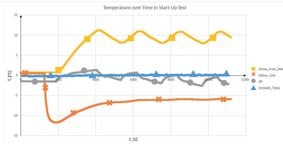
Figure 28: Data from test x, SCC is applied.
