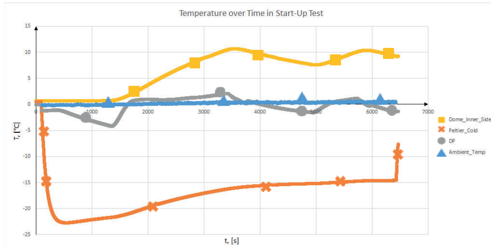
Figure 32: Data from test 4, SCC is applied.
