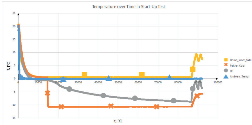
Figure 38: Data from test 7, SCC is applied.
