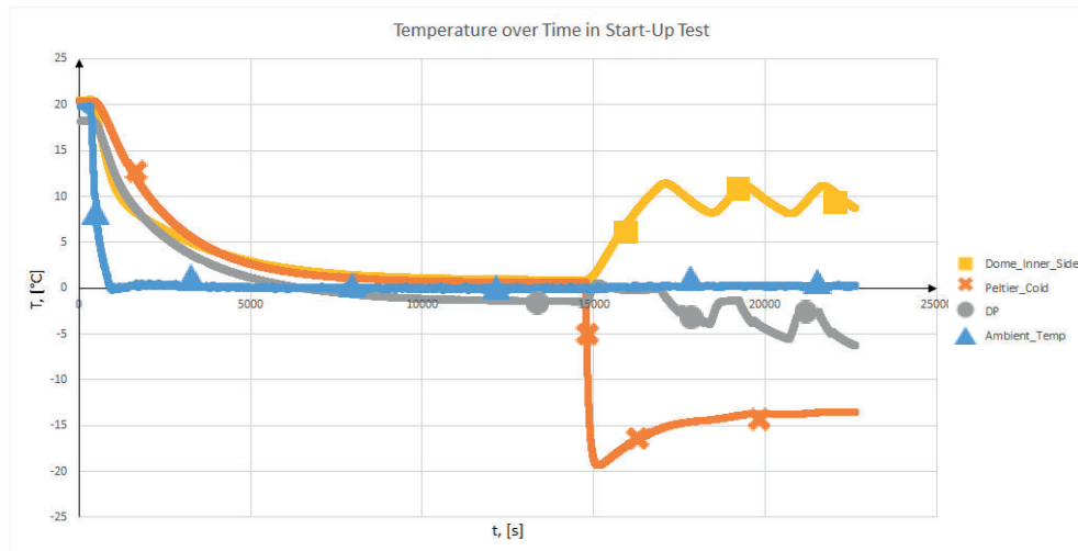
Figure 26: Data from test 1, SCC is applied.
