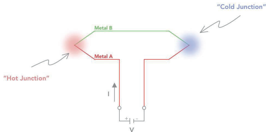
Figure 4: A demonstration of the Peltier effect.
