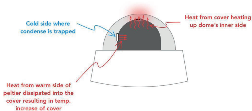
Figure 14: Demonstration of the idea with placement test
