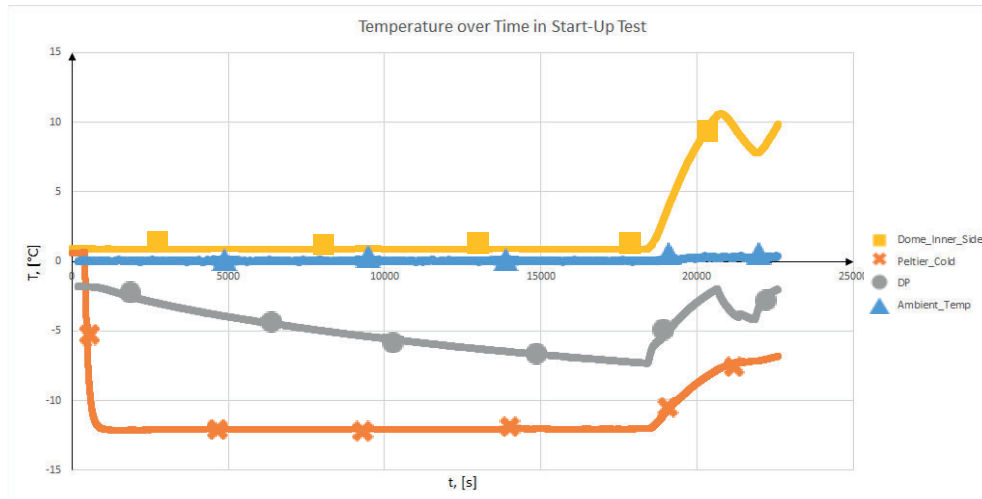
Figure 34: Data from test 5, SCC is applied.
