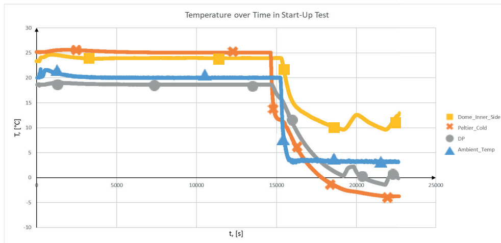
Figure 24 Data from test 5, SCC is applied.
