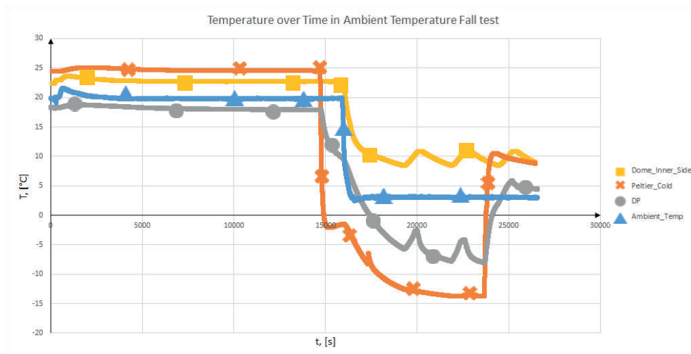
Figure 18: Data from test 2, SCC is applied.
