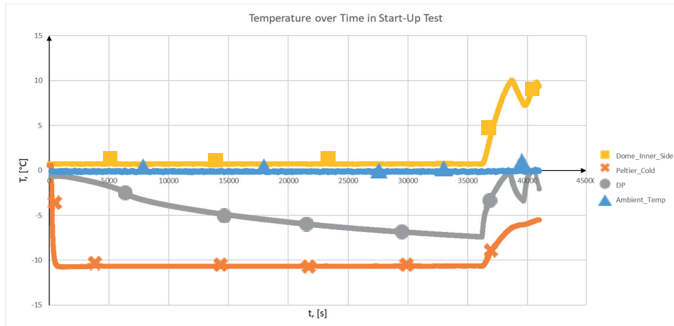
Figure 36: Data from test x, SCC is applied.
