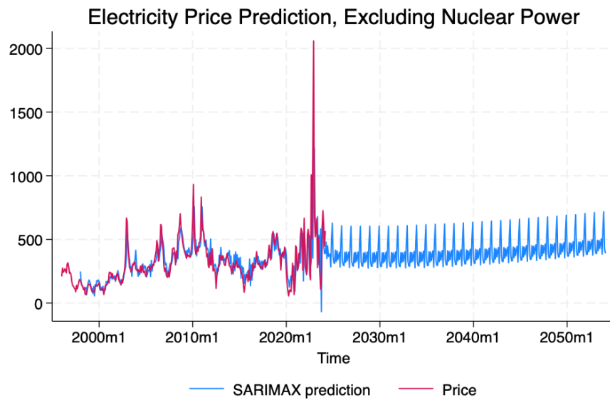
Figure A11. SARIMAX(2,0,2) \times (1,1,1)_{12} prediction excluding nuclear power.
