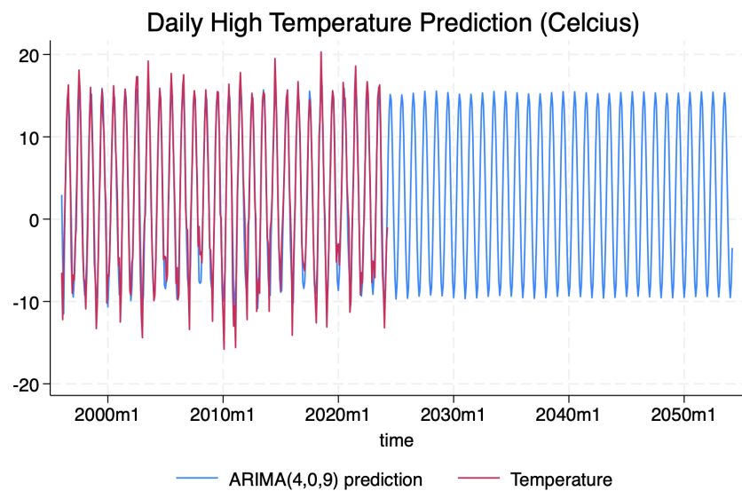
Figure A9. Predicted daily high temperature
