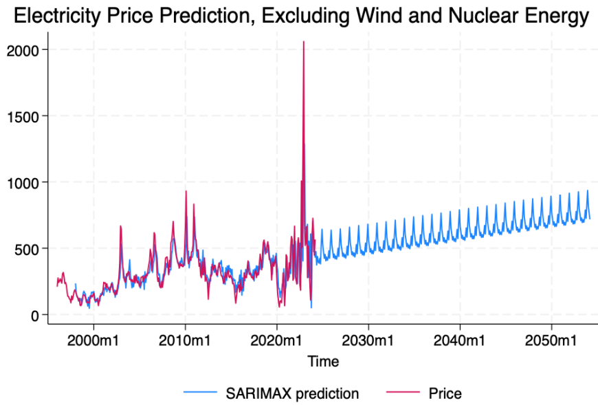
Figure A10. SARIMAX(2,0,2) \times (1,1,1)_{12} prediction excluding wind and nuclear power.
