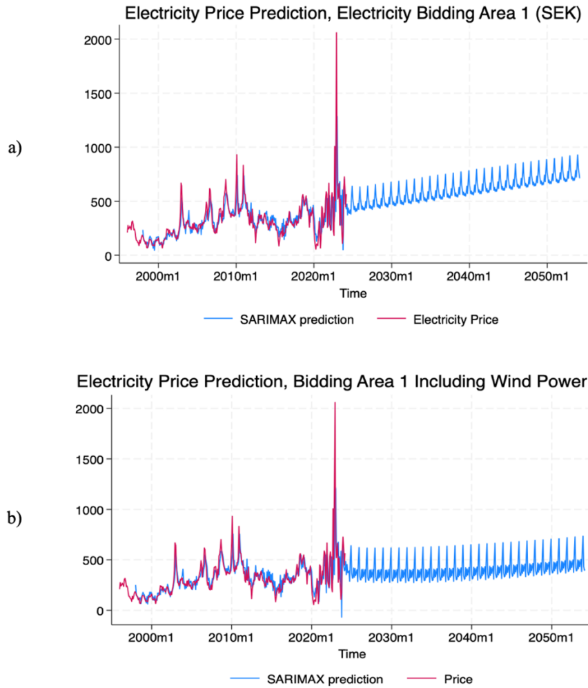
Figure 2. SEI Electricity Price Prediction (a) SARIMAX(2,0,2)x(1,1,1) 12 prediction excluding wind power as an exogenous variable. This model will be referred to as Scenario 1. b) SARIMAX(2,0,2)x(1,1,1) 12 prediction including the wind power prediction as an exogenous variable. This model will be referred to as Scenario 2.
