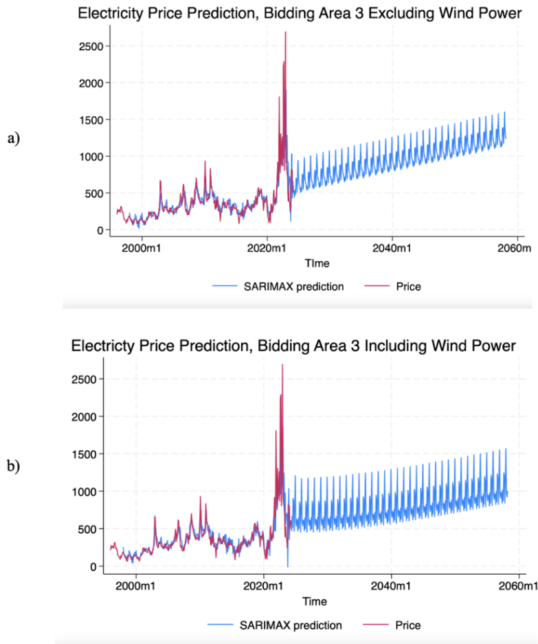
Figure 3. SE3 Electricity Price Prediction a) SARIMAX(2,0,2)x(1,1,1) 12 prediction excluding wind power as an exogenous variable, i.e. scenario 1, using Bidding Area 3 prices. b) SARIMAX(2,0,2)x(1,1,1) 12 prediction including wind power as an exogenous variable, i.e. scenario 2, using Bidding Area 3 prices.
