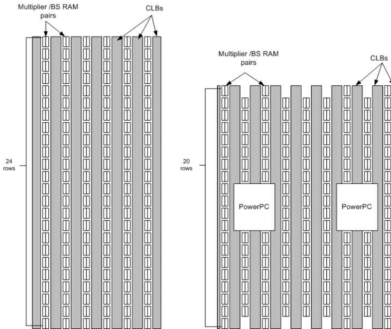
Figure 4.1 The configuration of a Virtex-II 6000 (left) and Virtex-II Pro P30 (right) from Xilinx. Grey columns represent bundling logic in form of CLBs, while the vertical boxes represent pairs of multiplier and BRAM macros. The placement of PowerPCs disturbs the matrix-style in the Pro P30 device.
