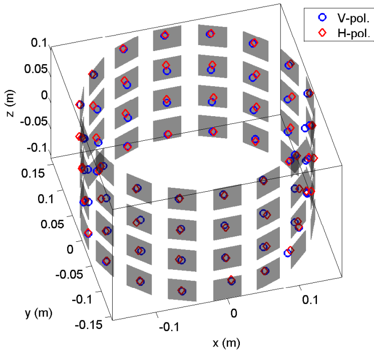
Figure 5.5: The RxPUC geometry with marked phase centers estimated from measured patterns.
