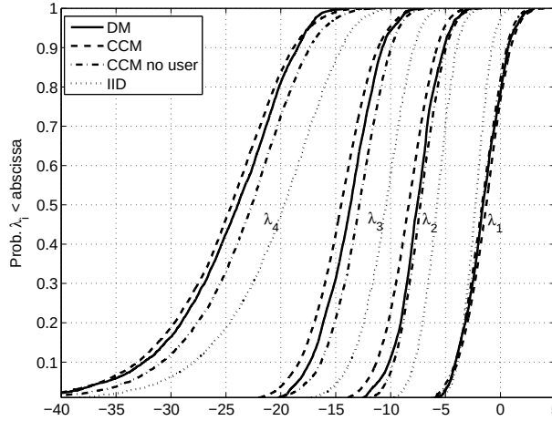
Figure 7: Ordered eigenvalue distribution of a 4 \times 4 channel for direct measured (DM), and CCM with and without phantom in talk mode (Scenario 2). For comparison the distribution for an i.i.d. complex Gaussian channel is shown.
