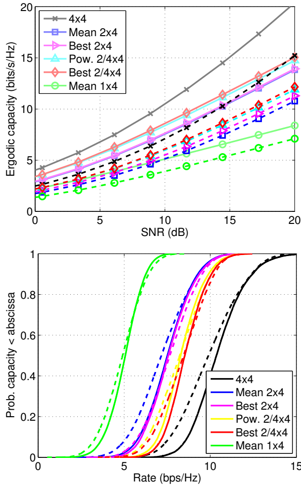
Figure 4: Ergodic capacity vs. SNR (top) and outage capacity distribution (bottom) at SNR=10dB for different MIMO systems with (dashed) and without (solid) user phantom present.
