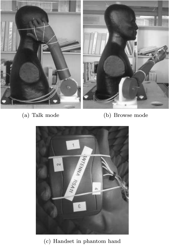
Figure 1: The user phantom in talk mode and in browse mode, and the four-antenna handset mock-up at one position inside the phantom hand.
