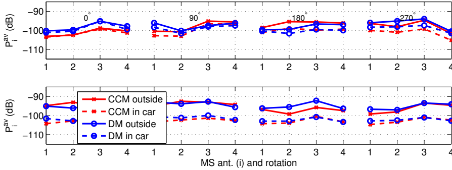
Figure 5: Average received signal powers of individual antenna elements of the phantom user with the smartphone mock-up for vertical polarization at the BS. The upper graph show the result in Scenario A and the lower in Scenario B.
