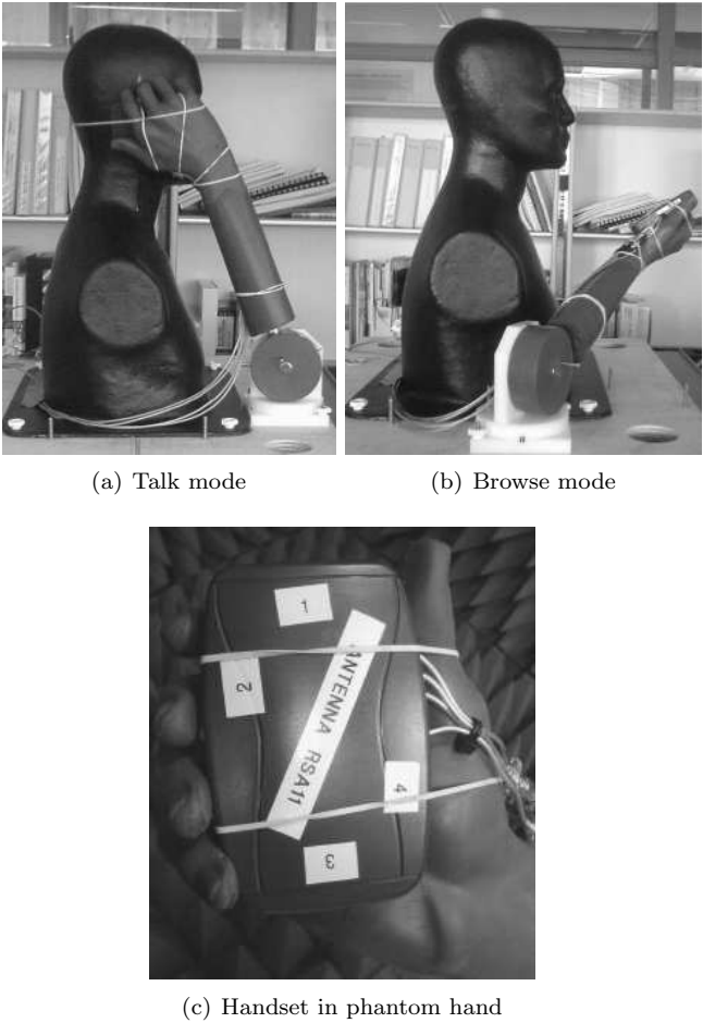
Figure 1: The user phantom in talk mode and in browse mode, and the four-antenna handset mock-up at one position inside the phantom hand.
