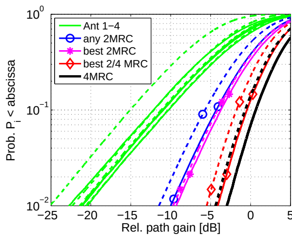
(b) Talk mode
