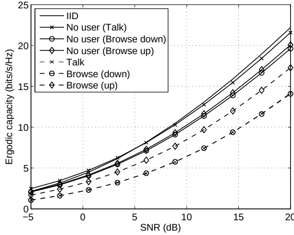
Figure 10: Ergodic capacity for a 4 \times 4 system, with waterfilling for Scenario 2. Results with and without phantom present are shown for the three user modes.
