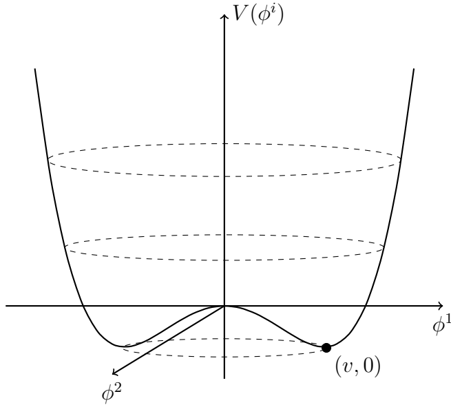
Figure 1.2: The linear sigma model potential V = -\mu^2(\phi^i)^2 + \lambda((\phi^i)^2)^2 , for N = 2 , plotted against the fields \phi^{1,2} . The infinitely degenerate vacuum states lie along the circle with radius \mu^2/\lambda = v , among them our choice of ground state (v, 0) .
