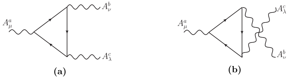
Figure 2.1: The triangle diagrams which spoil gauge invariance for chiral theories [13].
