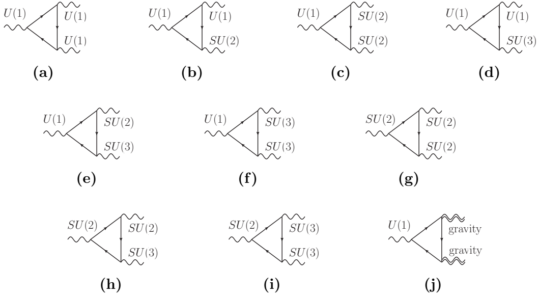
Figure 2.2: The complete set of potentially anomalous triangle diagrams.
