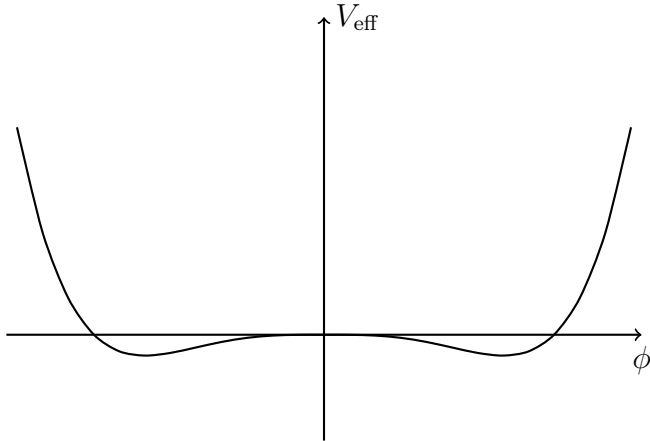
Figure 1.1: The function V_{\text{eff}} = a\phi^4 + b\phi^4 \log(\phi^2) , for some constants a, b , plotted against \phi . This function is of the form of the effective potential in Eqn. (1.11). The two minima are generated by quantum corrections, and spontaneously break the original reflection symmetry of the theory, despite the lack of a classical \mu^2 term.
