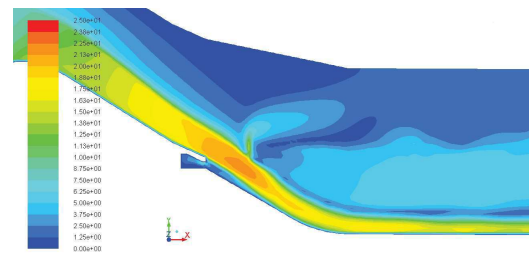
FIGURE 6.8: Velocity magnitude on the chute (3D- 1900m^3/s )
