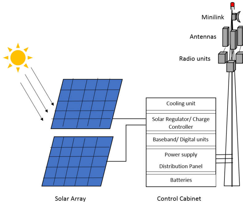
Figure 5.5: Overall design of a solar powered RBS.
