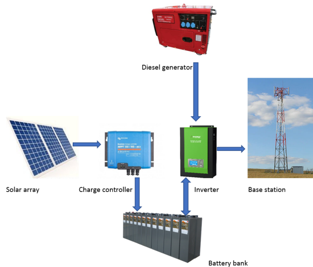
Figure 5.13: Solar diesel hybrid site set up
