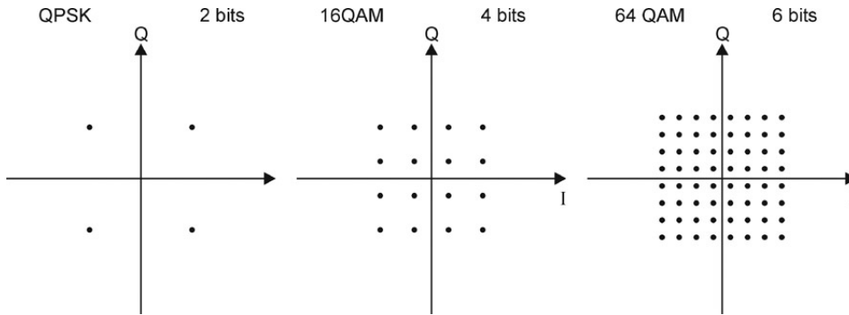
Figure 1.4: Modulation scheme for QPSK, 16-QAM and 64-QAM. The angle and absolute value of the points corresponds to phase and amplitude of the wave [4].
