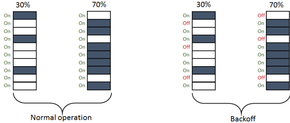
Figure 4.1: Overview of an example with 10 resource blocks in frequency domain. In normal operation all PAs are biased, showed as "On" in the image. With backoff to the right there is a limit on the number of biased PAs and some are unbiased, showed as "Off". In this example the throughput is limited to 70% of its original value. This backoff can be used as an ECO-mode.
