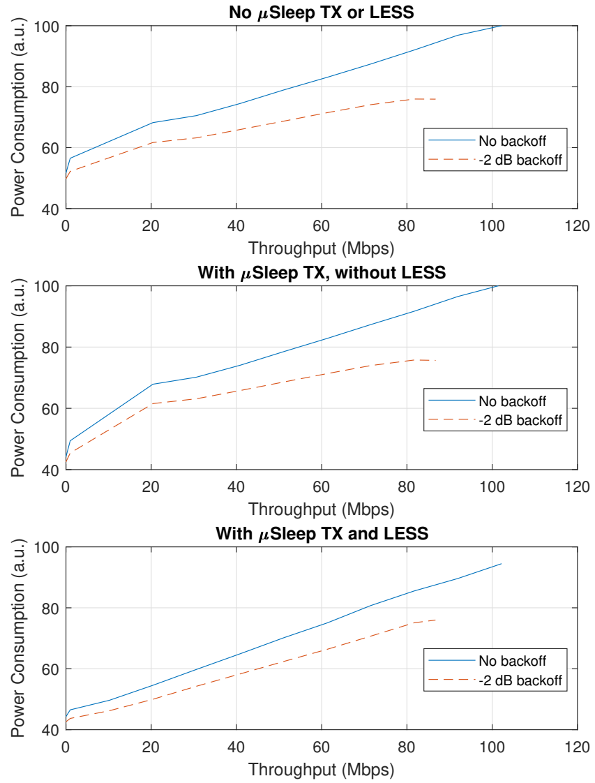
Figure 4.9: Power savings from the ECO-mode in a radio B. The graphs show scenarios with and without Micro Sleep TX and LESS.
