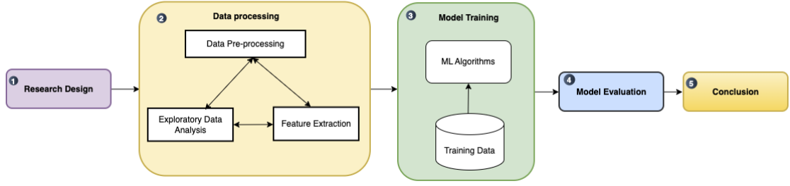
Figure 4.1: Research Method
