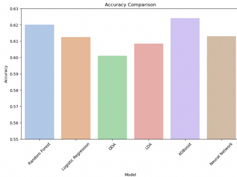
Figure 5.1: Accuracy Comparison
