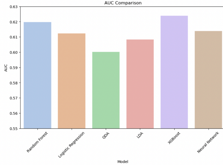
Figure 5.4: AUC Comparison
