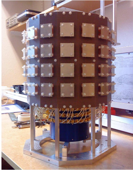
Figure 5.4: The RxPUCA antenna.
