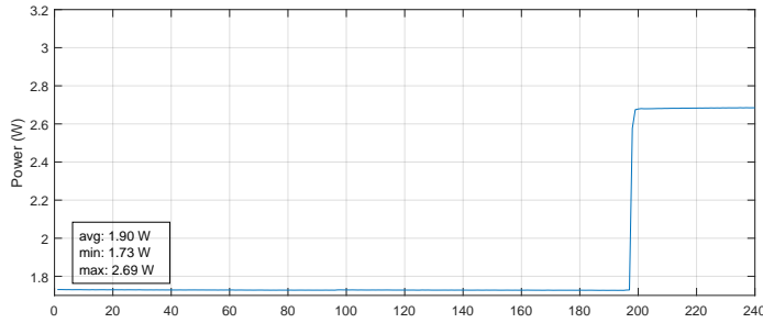
Figure 5.5: CPU suspend idle result.
