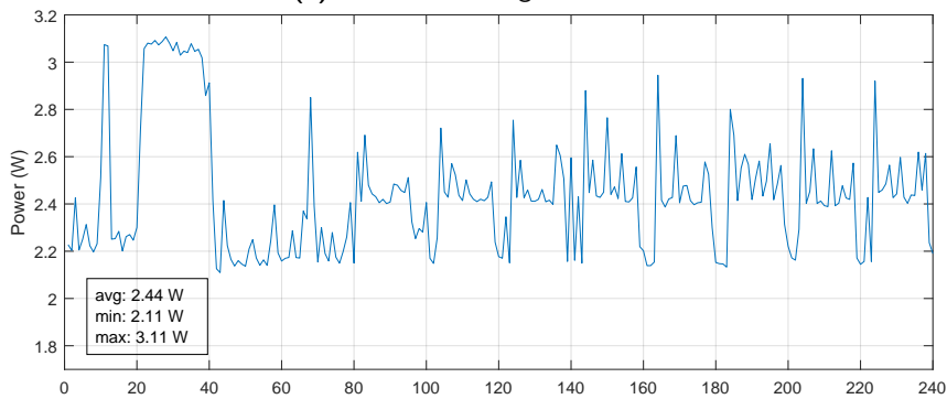
(c) CPUIdle + OSDP + JMeter.
