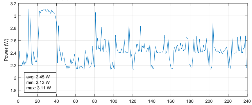
(c) CPUFreq + CPUIdle + OSDP + JMeter.
