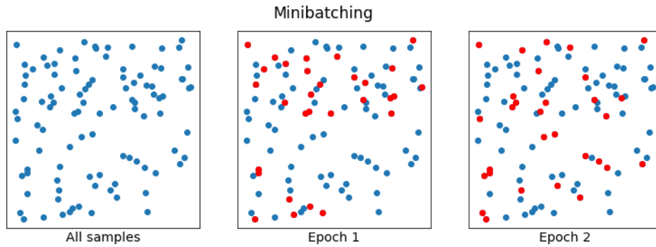
Figure 2.1: In a set of 100 samples a random mini-batch of 30 samples is selected in the first epoch. In the next epoch a new mini-batch is randomly selected.
