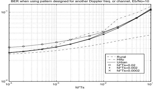
Fig. 7 Changes in the bit error rate due to Doppler mismatch and power delay profile mismatch. The pilot patterns designed for f_d T_s = 0.02 , 0.002 and 0.0002 were used at different Doppler values and the designed patterns for typical urban environment were used in hilly terrain and rural area.
