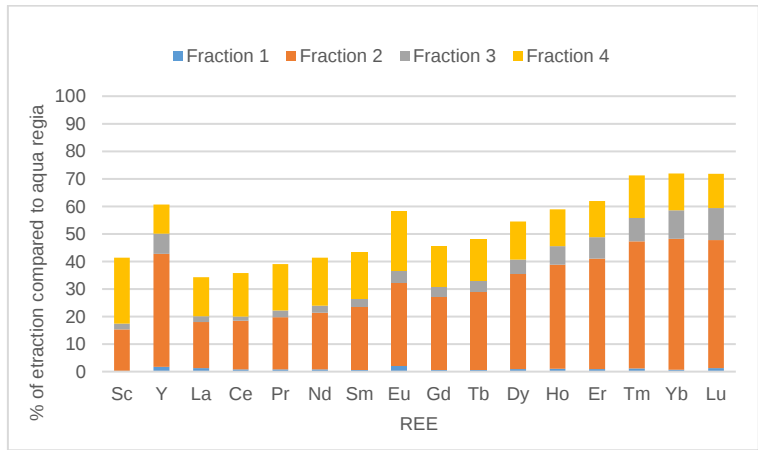
Figure 7: Sequential extraction of REE in ESS soil samples a) E4, b) E258 (where Eu in the fraction 4 was an outlier), c) E331, d) E344 using the 4-step Mittermüller et al. method [67] (see section 4.4.2 for the detailed methods)
