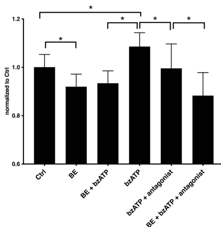
Fig. 24 Effect of bilberry extract (BE) on endothelial vesiculation. BE incubation significantly decreased vesicle release and bzATP increased the vesiculation compared to the control cells. Pre-incubation with BE prevented bz-ATP evoked vesiculation. Mean ± SD. One-way ANOVA with FDR correction of Benjamini and Hochberg. *Statistically significant, p < 0.05 .
