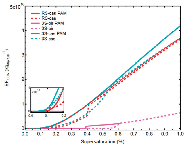
Figure 14: Results from paper v, comparing freshly emitted and aged emissions from a subset of stove-fuel combinations: Rocket stove and casuarina logs (RS-cas); Three-stone stove and casuarina logs (3S-cas); and three-stone stove with birch logs (3S-bir). Original caption: Examples of emission factors of CCN as estimated for the aerosol photochemically aged inside PAM with the fresh emission factors included for comparison. For the 3S-cas PAM experiment, the nucleation particle mode grew large enough to dominate near a mobility diameter of 65 nm, which resulted in an increase in CCN for high supersaturations.
