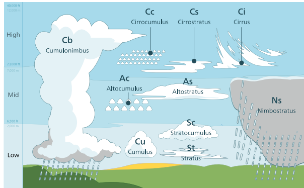
Figure 4: The ten genera of cloud types commonly associated with the troposphere. Author: Valentin de Bruyn. Licenced under Creative Commons CC-BY-SA 3.0 ( https://creativecommons.org/licenses/by-sa/3.0/ ).
