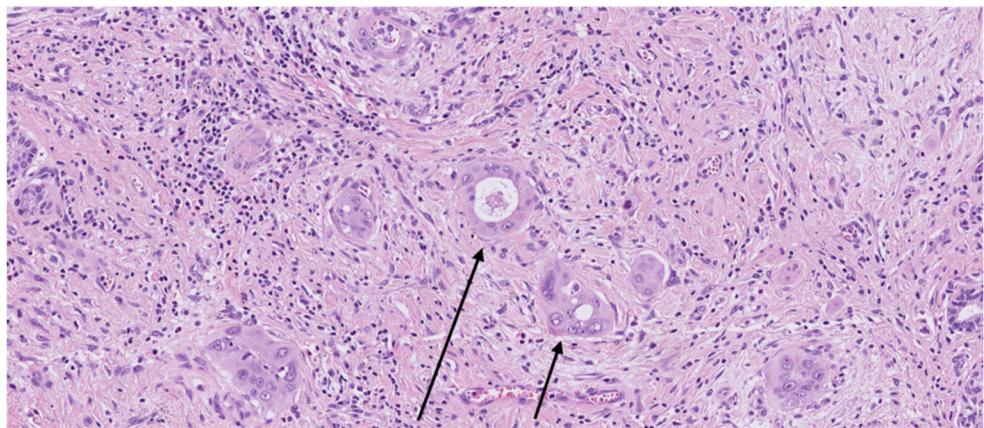
Figure 2. Macroscopic picture of a distal cholangiocarcinoma from serial axial sections through the pancreatic head and microscopic pictures from the same patient showing a poorly differentiated adenocarcinoma originating from the common bile duct with an ample desmoplastic reaction. Image courtesy of Dr Agata Sasor.
