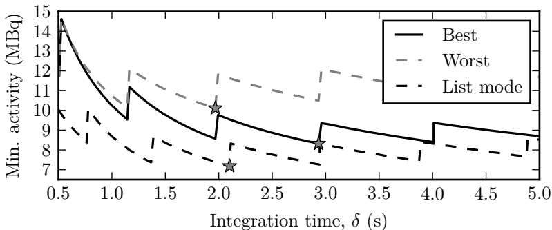
Figure 2.16: An example of a plot showing the minimum detectable activity for a specific radionuclide given a specific set of measurement parameters when performing a mobile survey. The stars indicate the lowest valley for each curve and thus the optimal integration time and minimum detectable activity. Adaptation of a figure shown in Paper V.
