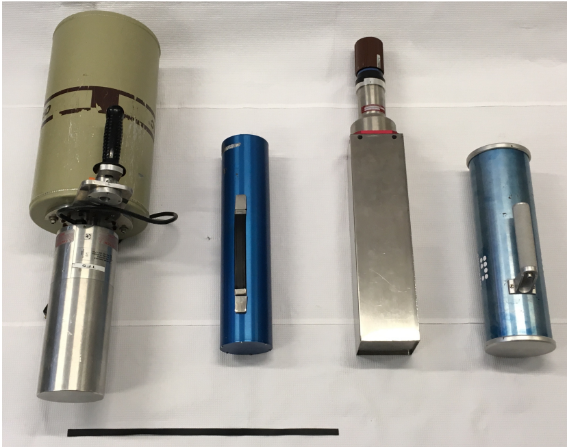
Figure 3.1: The four gamma spectrometry systems used in the research presented here. From left to right: 1. HPGe, 2. \text{Ø}7.6 by 7.6\text{cm}^3 NaI(Tl), 3. 4 l NaI(Tl) 4. LaBr 3 :Ce. Note that the 4 l NaI(Tl) detector has been removed from its outer container. The black ruler in the foreground has a length of 50 cm.
