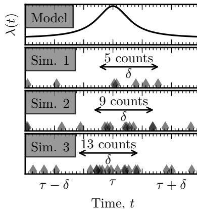
Figure 2.15: The top panel represents the distribution that describes the probability of a moving detector detecting radiation from a stationary source (see Figure 2.13). The next three panels illustrate simulated measurements and the maximum number of counts achieved using an integration time of 1 s. Adaptation of a figure shown in Paper V.
