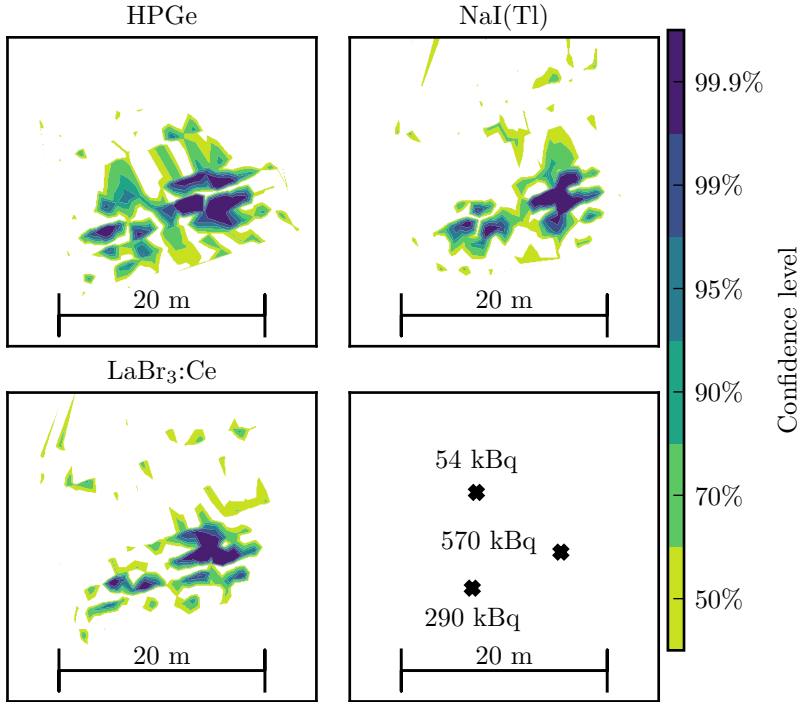
Figure 4.2: The areas in which ^{137}\text{Cs} sources were detected with 50–99.9% confidence (true positive probability) when surveyed using a HPGe, NaI(Tl) and LaBr 3 :Ce detector. Surface areas are given in Table 4.1. Note that the lower right figure illustrate the actual locations and activities of the ^{137}\text{Cs} sources. Based on data published in Paper II.
