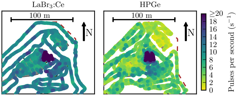
Figure 4.3: Total number of pulses in the ^{137}\text{Cs} region of interest when surveying a radioactive waste repository using the HPGe detector and the \text{LaBr}_3:\text{Ce} detector. Due to the high pulse rate directly above the repository, the colour scale is limited to a maximum of 20 counts per second. Based on data published in Paper II.
