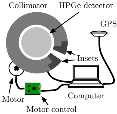
Figure 3.10: Overview of the subsystems of the collimator-based gamma radiation mapping system. Adaptation of a figure shown in Paper IV.
