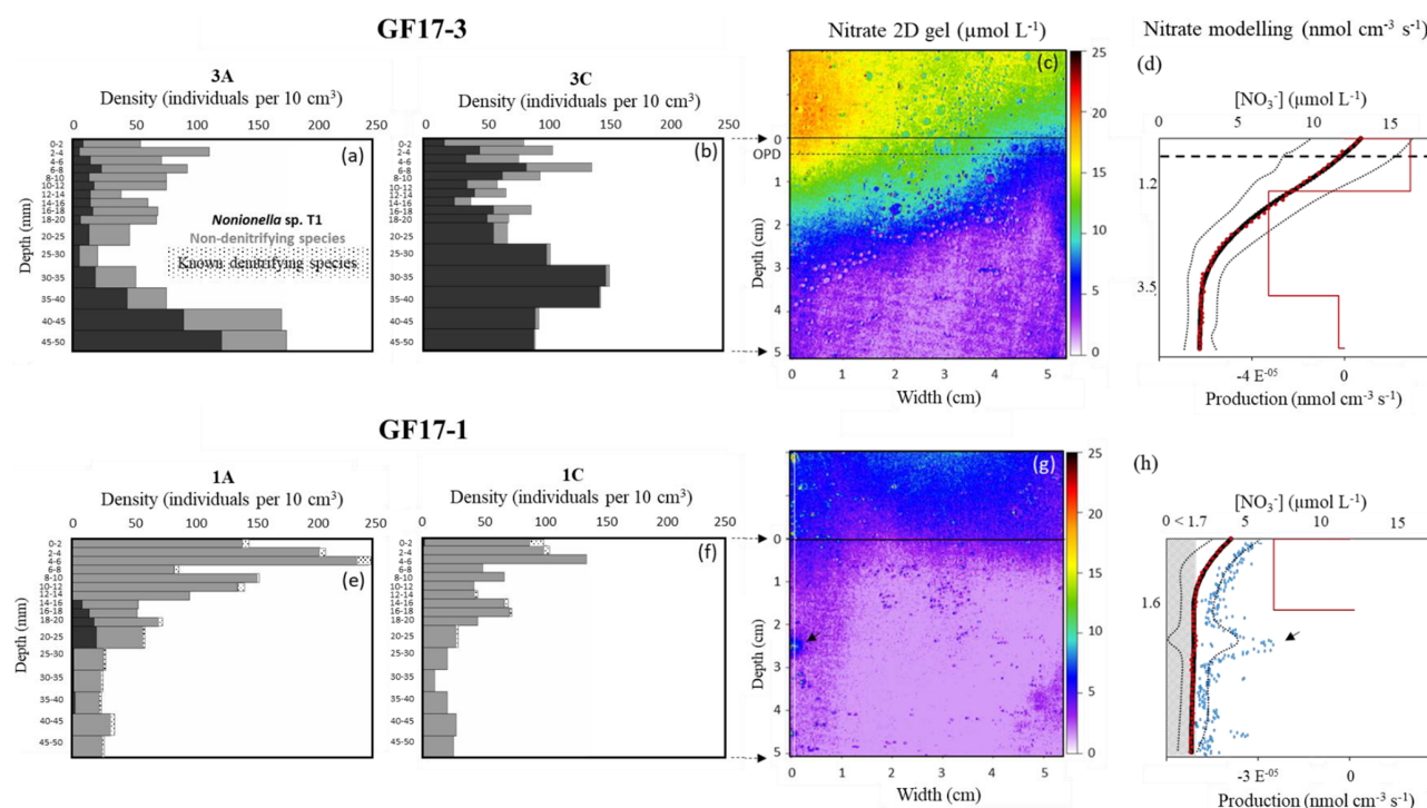
Figure 5. Micro-distributions of living-foraminifera densities in GF17-3 oxic station (a, b) and in GF17-1 hypoxic station (e, f). Nonionella sp. T1 specimens are in black, the sum of the non-denitrifying species is in grey and the small dots (e, f) show the other denitrifying species (known and potential candidates). The maps of porewater nitrate 2D gels are presented for stations GF17-3 (c) and GF17-1 (g). The SWI is represented by a black line at 0 cm depth (c, g), and the OPD (oxygen penetration depth) is represented by the dashed line in bold at 4.7 \pm 0.2 mm depth (c). Nitrate 1D profiles (d and h, black dots) are calculated using the average value of each pixel line of the nitrate distribution image (290 pixels wide); the SD is represented by two fine, dotted lines. The corresponding best-fitting concentration profiles (red dots, d and h) and the production zones (red line) are modeled with PROFILE software. The 1D profile corresponding to x = 1 mm (white line, g) is represented with a blue square profile (h), and the deep nitrate spot is indicated by a black arrow. The grey hatching zone (h) represents the detection limit of the nitrate 2D gel ( < 1.7 \mu\text{mol L}^{-1} ).
