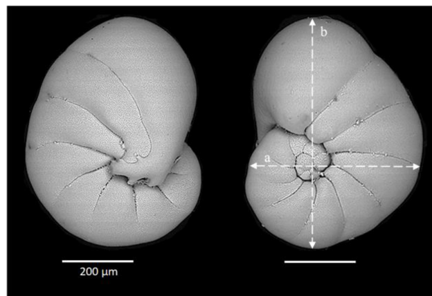
Figure 4. Scanning electronic microscope images of a Nonionella sp. T1 from the GF17-3 oxyc station in the Gullmar Fjord. White lines (labeled a and b) correspond to measured distances serving for a spheroid prolate volume model.
