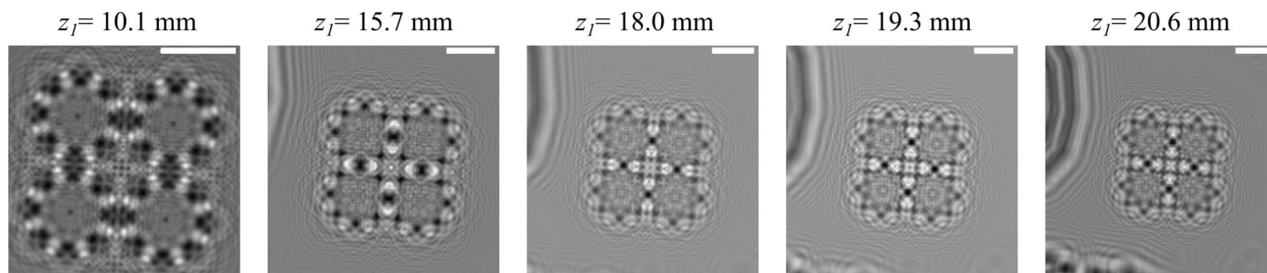
Figure 4 Recorded holograms at different defocusing distances ( z_I ) of the 2D test pattern. The white scale bar corresponds to 4 \mu\text{m} for all the images.
