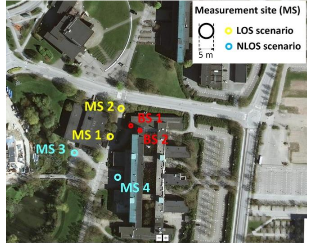
Fig. 1. Aerial photo of the outdoor measurement area. BS locations are indicated by labels BS 1 (low-roof) and BS 2 (high-roof). UE sites are labeled with MS 1 to MS 4, and the locations of the 5 m diameter circles have also been indicated. UE sites MS 1 and MS 2 have LOS condition to the BS, while MS 3 and MS 4 have NLOS.
