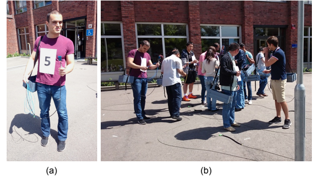
Fig. 2. (a) A user holding the MS user equipment antenna with an inclination of 45°. (b) Users moving randomly within the five-meter diameter circle at UE site MS 4.
