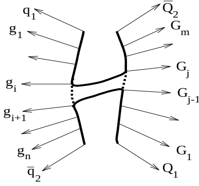
Figure 1: The gluons g_1 g_2 \dots g_n (with E > \Gamma_W ) are emitted from the original q_1 \bar{q}_2 pair while G_1 G_2 \dots G_m are emitted from the Q_1 \bar{Q}_2 pair. The two systems q_1 g_1 \dots g_i G_j \dots G_m \bar{Q}_2 and Q_1 G_1 \dots G_{j-1} g_{i+1} \dots g_n \bar{q}_2 are then colour singlets with probability 1/9 for each value of i and j . They may thus form independent hadron chains or strings.
