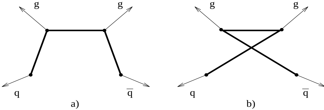
Figure 2: The production probability for a q\bar{q}gg state is, in perturbative QCD, larger for the colour connection which corresponds to a “shorter string” as in fig a).
