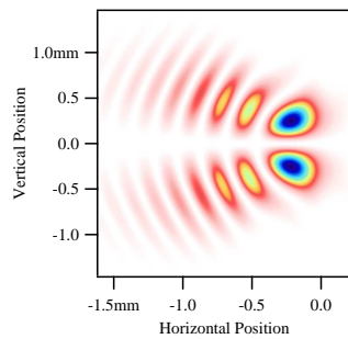
Figure 16. Image of \pi -polarized SR with depth-of-field characteristics. \alpha_H = 18 mrad and \lambda = 930 nm. FBSF calculated in SRW.
