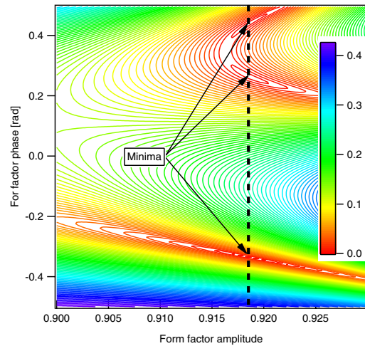
FIG. 13. Contour plot of the penalty function g for R_s = 4.4 \text{ M}\Omega and \Delta f = -60.36 \text{ kHz} . The origin of the phase coordinate is chosen such that V_{MC}(\varphi) = V_{\pi} \sin(\varphi + \varphi_s) . The vertical dashed line indicates the form factor amplitude value corresponding to all three minima.
