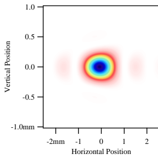
Figure 12. Image of \sigma -polarized SR with Fraunhofer diffraction characteristics. \alpha_H = 2 mrad and \lambda = 930 nm. FBSF calculated in SRW.
