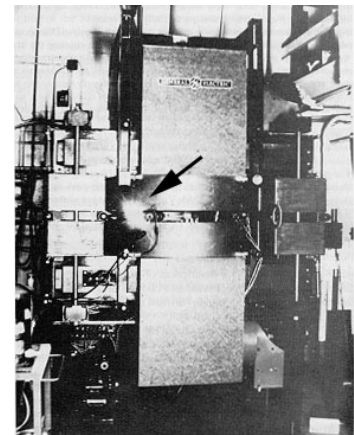
Figure 1. Photograph of SR from the General Electric 70 MeV synchrotron. The arrow indicates the bright spot between the magnets.
