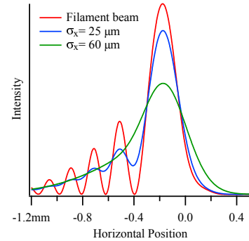
Figure 18 d). a_H = 18 \text{ mrad} , \lambda = 930 \text{ nm} . Beam size determination at \sigma_x \approx 25 \mu\text{m} by fringe contrast.
