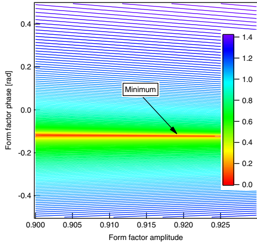
FIG. 14. Contour plot of the penalty function g for R_s = 4.4 M \Omega and \Delta f = -60.36 kHz. The origin of the phase coordinate is chosen such that V_{MC}(\varphi) = V_{rf} \sin \varphi .
