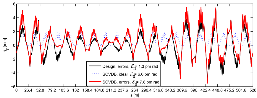
(b) Resulting vertical emittance, \mathcal{E}_{II} = 8 \text{ pm rad} scaling.
