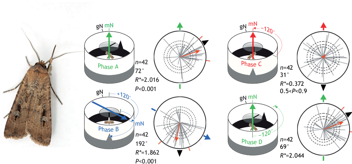
Fig. 4. Migratory orientation in Bogong moths is multimodal. Individual moths were tethered at the center of a cylindrical Perspex flight arena placed vertically on a table outdoors. Moths were then attached to the end of a vertical shaft connected to an encoder that continuously measured the instantaneous orientations of steadily flying moths that were free to turn in any azimuthal direction. Each moth was then subjected to magnetic and visual cues during four 5 min phases (A–D) and their directions and directedness (orientation and length, respectively, of gray vectors in circular plots) measured. When the positions of the magnetic field (thick colored arrows) and visual landmarks (black triangular ‘mountain’ and dorsal stripe) are correlated and turned together (phases A, B and D), the moth population (gray vectors, n=42 ) remains significantly oriented near the landmarks (as indicated by the long (highly directed) red population mean vectors; P<0.001 ). When the two cues are set in conflict (phase C), moths become disoriented [as indicated by the short (undirected) red population mean vector; 0.5<P<0.9 ]. The directedness (length) of the population mean vector is given by its R^* value: the greater the R^* value, the more directed the population of moths it represents. The R^* value also reveals the likelihood that the mean flight direction of a population of moths – where each moth has its own direction and directedness (direction and length of gray vectors) – differs significantly from a random, undirected population (according to Moore’s modified Rayleigh test: Moore, 1980). Dashed circles: required R^* value for statistical significance (i.e. the R^* value required to reliably distinguish the directedness of the population from a random, undirected population): P<0.05 , P<0.01 and P<0.001 , respectively, for increasing radius. Outer radius of plots: R^*=2.5 . Red radial dashes: 95% confidence interval. gN, geographic north. mN, magnetic north. Data are from Dreyer et al., 2018.
