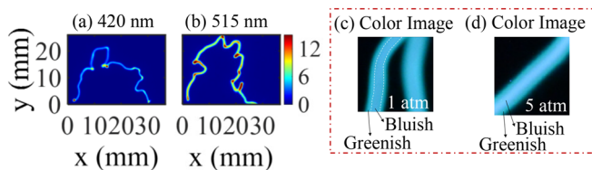
FIG. 8. Imaging of plasma columns in the Ar-0.1%CH 4 mixture. (a) and (b) are captured by the ICCD camera with a gate width of 30 μs; (c) and (d) are color images captured by the Nikon digital camera with an exposure time of 1/8000 s.
