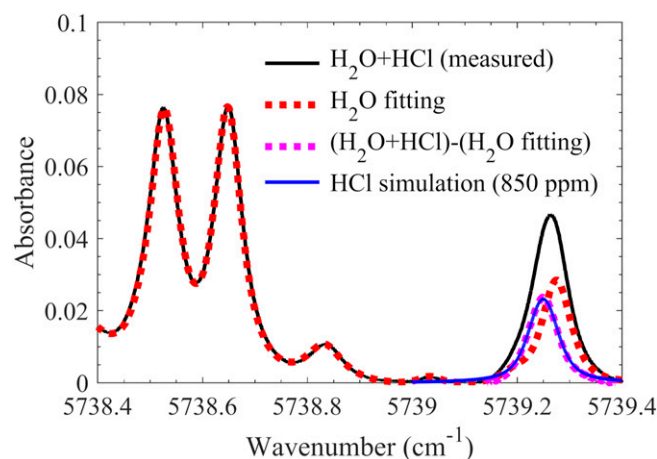
Figure 6. Absorbance spectrum obtained in the hot flue gas at 1540 K with 830 ppm Cl seeding (black line), the \text{H}_2\text{O} absorbance spectrum fitted by the \text{H}_2\text{O} spectra of our database at 1540 K (red dot line), the HCl absorption obtained after the subtraction of the water absorption (magenta dot line) and the corresponding fitting of 850 ppm HCl using HITRAN2016 database (blue line).
