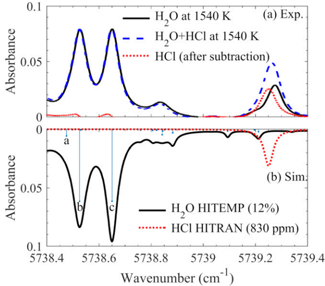
Figure 3. High resolution absorbance spectra of H 2 O and HCl measured in hot flue gas ( T = 1540 K) provided by flame F7 (a), and the calculated ones of 12% H 2 O and 830 ppm HCl at 1540 K (b) using HITEMP2010 and HITRAN2016 database, respectively.
