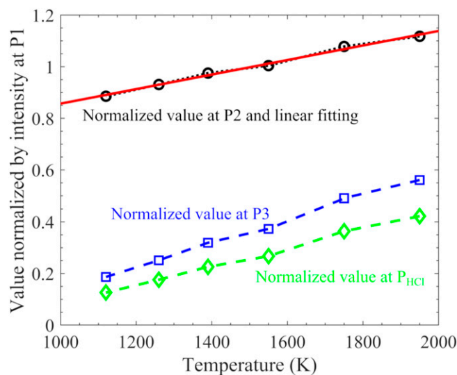
Figure 5. Normalized absorbance at position P2, P3, and P_{\text{HCl}} (as marked in Fig. 4), as a function of temperature, and corresponding linear fitting used for temperature estimation.
