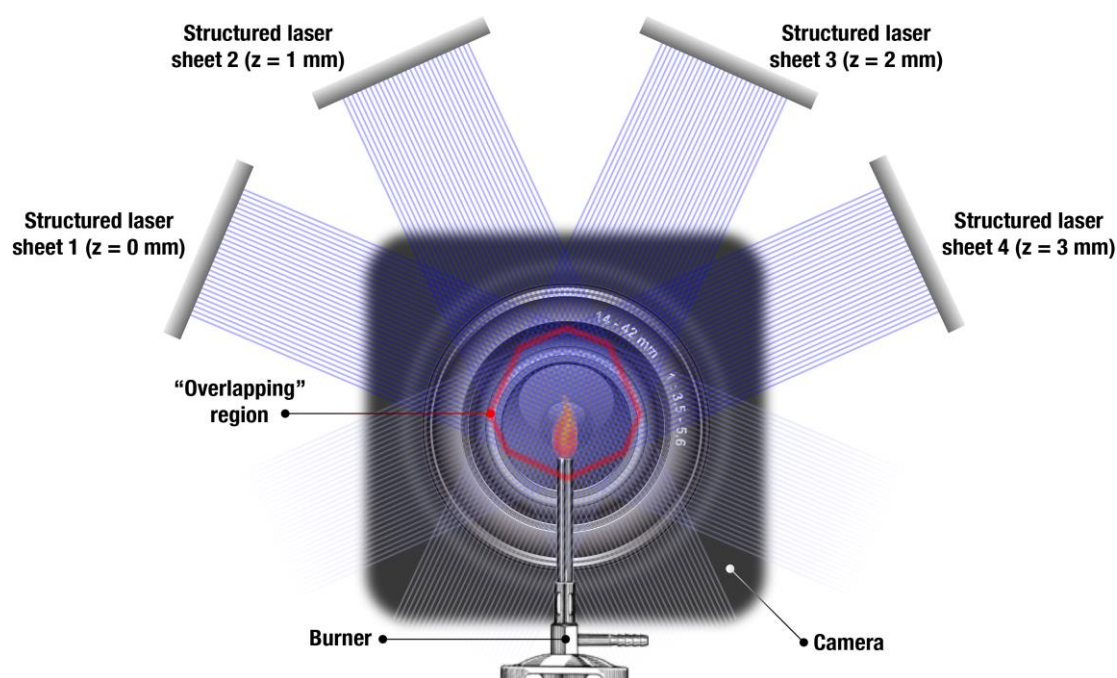
Figure 3. Schematic of the optical configuration. The four structured laser sheets arrive at different angles (approximately 20°, 65°, 115°, 160°), effectively placing the respective signals at different locations in reciprocal space. The spatial frequency of the superimposed intensity modulation was approximately 5 lp/mm.
