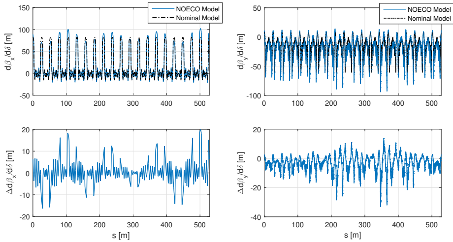
Figure 4.8: Horizontal (left) and vertical (right) chromatic functions and their errors relative to the chromatic functions of the design lattice.
