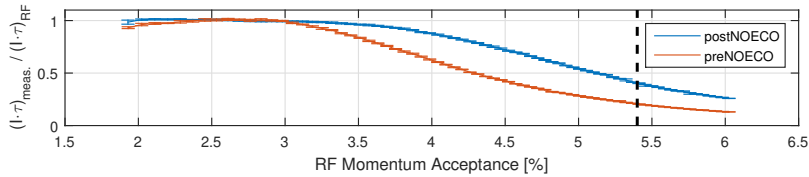
Figure 4.20: Measured current-lifetime product plotted against RF momentum acceptance as a ratio of measured current-lifetime product to simulated Touschek lifetime only determined by the RF momentum acceptance. The vertical dashed line corresponds to the RF momentum acceptance of the MAX IV 3 GeV ring during delivery at the time of the measurements. At this acceptance value the NOECO symmetrization increased the Touschek lifetime by a factor of 2.
