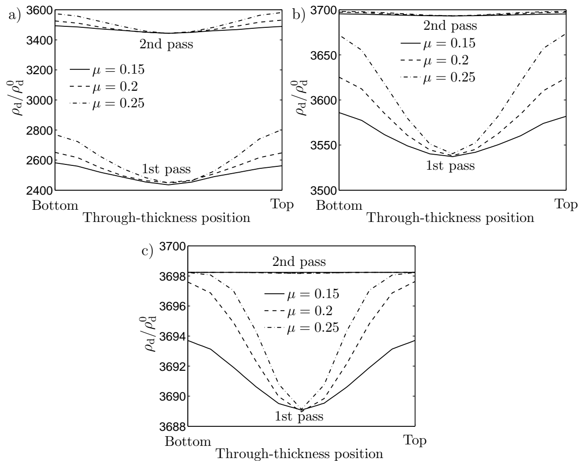
Figure 7: Influence of level of friction between sheet and rollers on the through-thickness variation of the normalized dislocation density in the sheet after one and two rolling passes, respectively. Results are obtained at thickness reductions (per pass) of: (a) 20 %, (b) 40 % and (c) 60 %.
