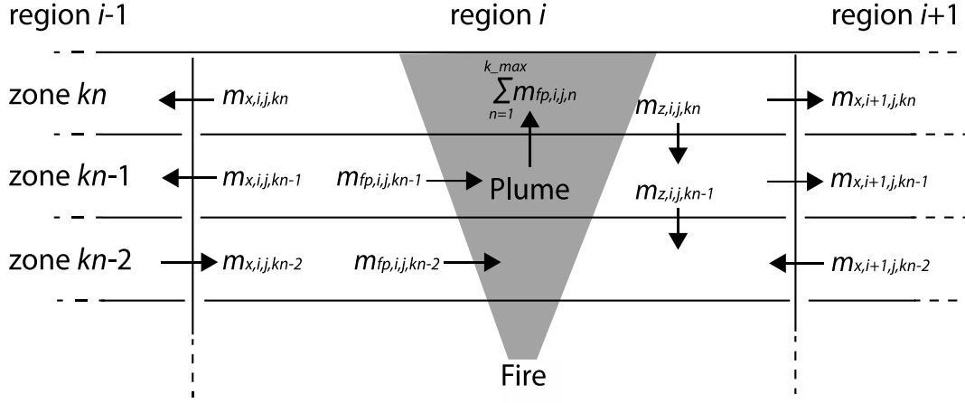
Figure 1: Principles of the multi-zone concept, re-drawn from Suzuki et al (2004).
