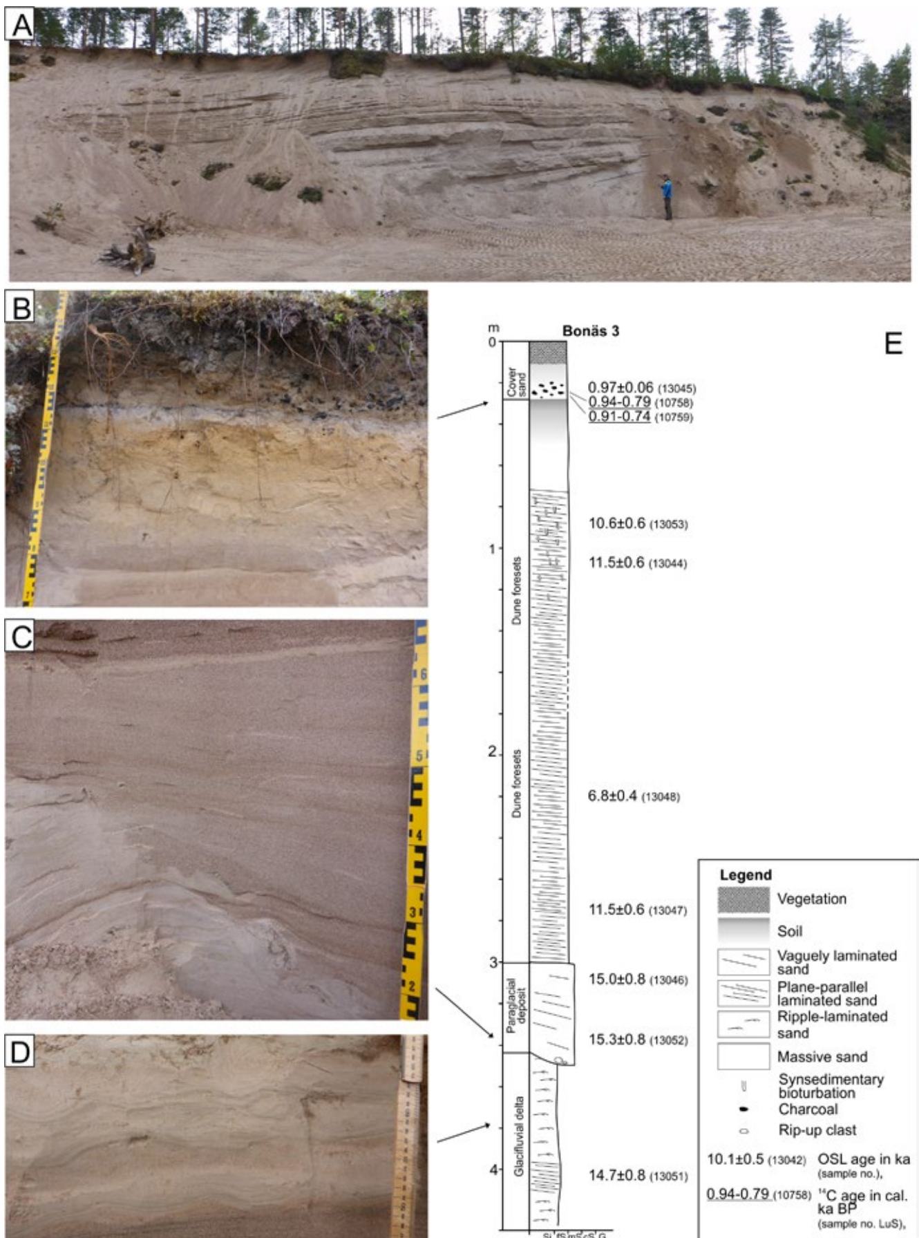
Fig. 12. Bonäs 3 (61.100°N, 14.470°E) is one of our key sites in Dalarna. Here glaciﬂuvial, paraglacial, dune/interdune sand and coversand are found in superposition. A. Overview of the exposure in the sandpit. B. Present soil and a palaeosol in the uppermost part of the section. C. Erosional boundary between glaciﬂuvial (light grey, lower left) and paraglacial (light brown, upper right) deposits. D. Glaciﬂuvial ripple-laminated sand. E. Composite log (modified from Alexanderson & Bernhardson, in press).
