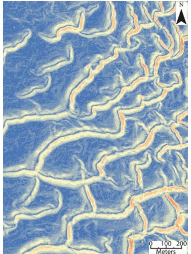
Fig. 8. Slope raster image of part of Bonäsheden (© Lantmäteriet, i2012/927). Blue shows a low slope angle, while yellow and red show a steeper slope angle. The steeper lee sides facing SE are clearly distinguished in this type of image.
