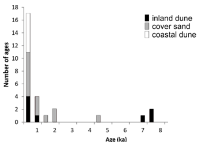
Fig. 33. Histogram of ages (OSL, C14) younger than 8 ka classified by origin: inland dune, coversand and coastal dune.
