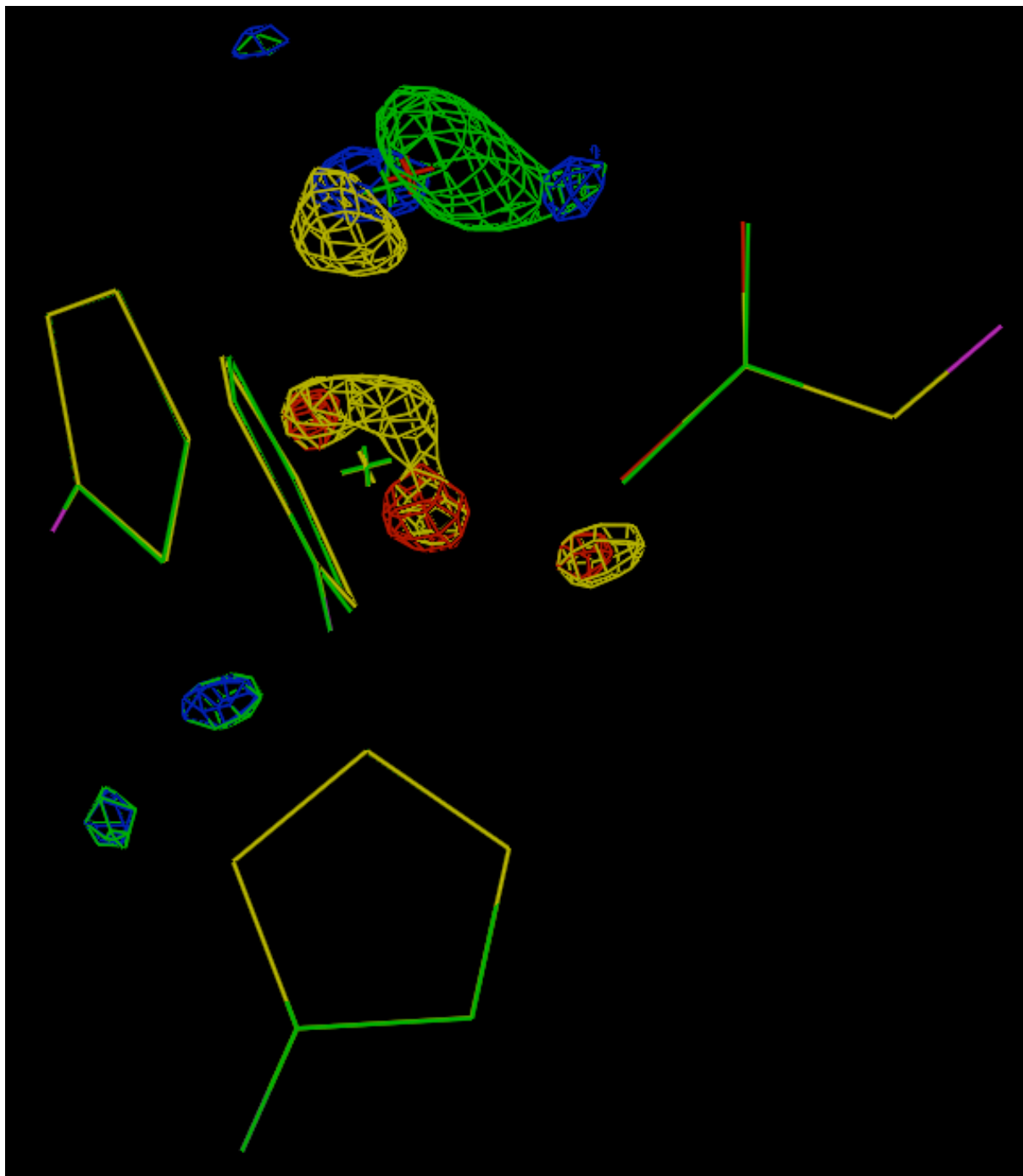
Figure 2. A comparison of the quantum refined OH - (green) and water (red/yellow/magenta) structures in the reduced protein (the two structures superimpose to a large extent). The Mn ion is marked by a green or yellow cross near the centre of the figure. The oxygen atom of the ligand is a green or red cross in the top of the figure. His-26 (bottom), His-171 (left), His-81 (almost from the side of the imidazole ring), and Asp-167 (right) are also included. The figure also shows the f_o - f_c difference maps of the two structures at the 3.5 \sigma level: blue (positive) and red (negative) for the water structure and green (positive) and yellow (negative) for OH - structure.
