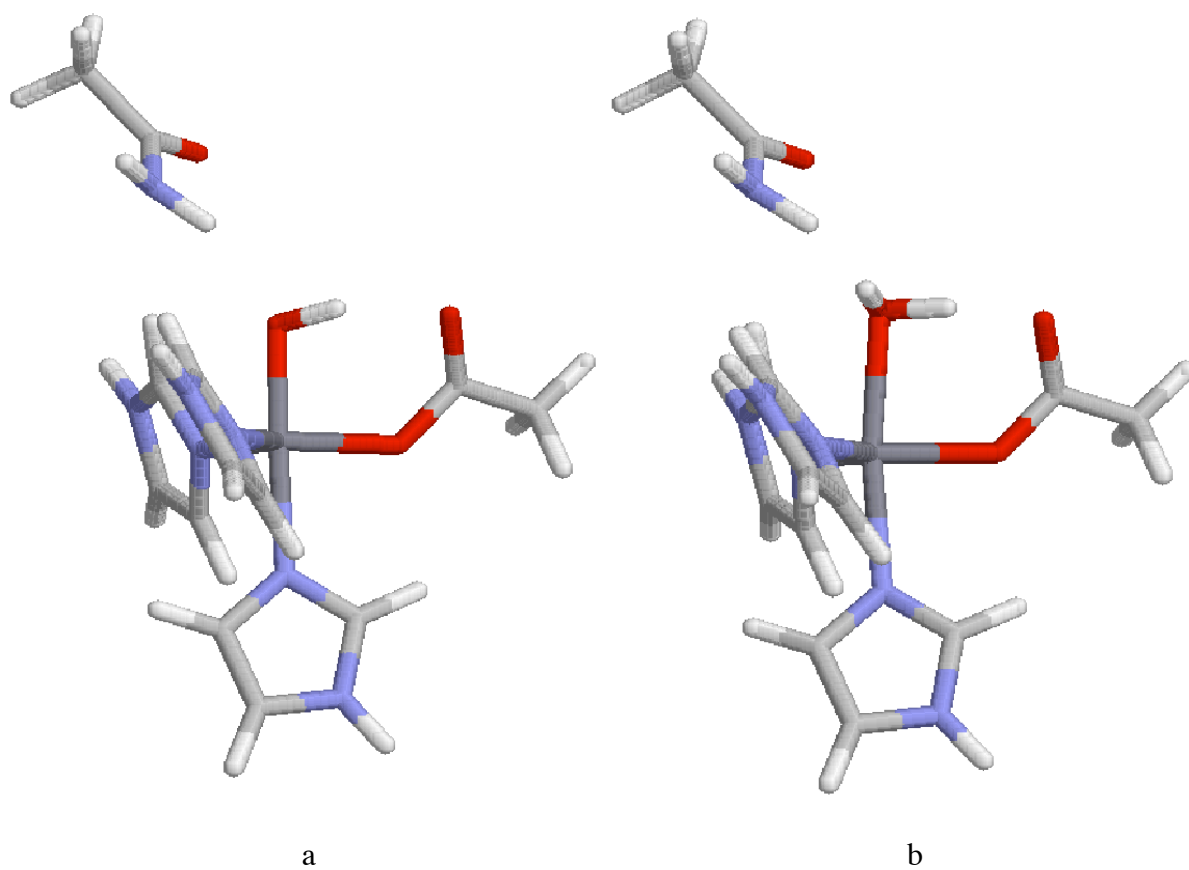
Figure 4. The structure of the quantum system in the quantum refined structures of (a) the oxidised structure with \text{Mn}^{3+}\text{-OH}^- (b) and the reduced structure with \text{Mn}^{2+}\text{-H}_2\text{O} .
