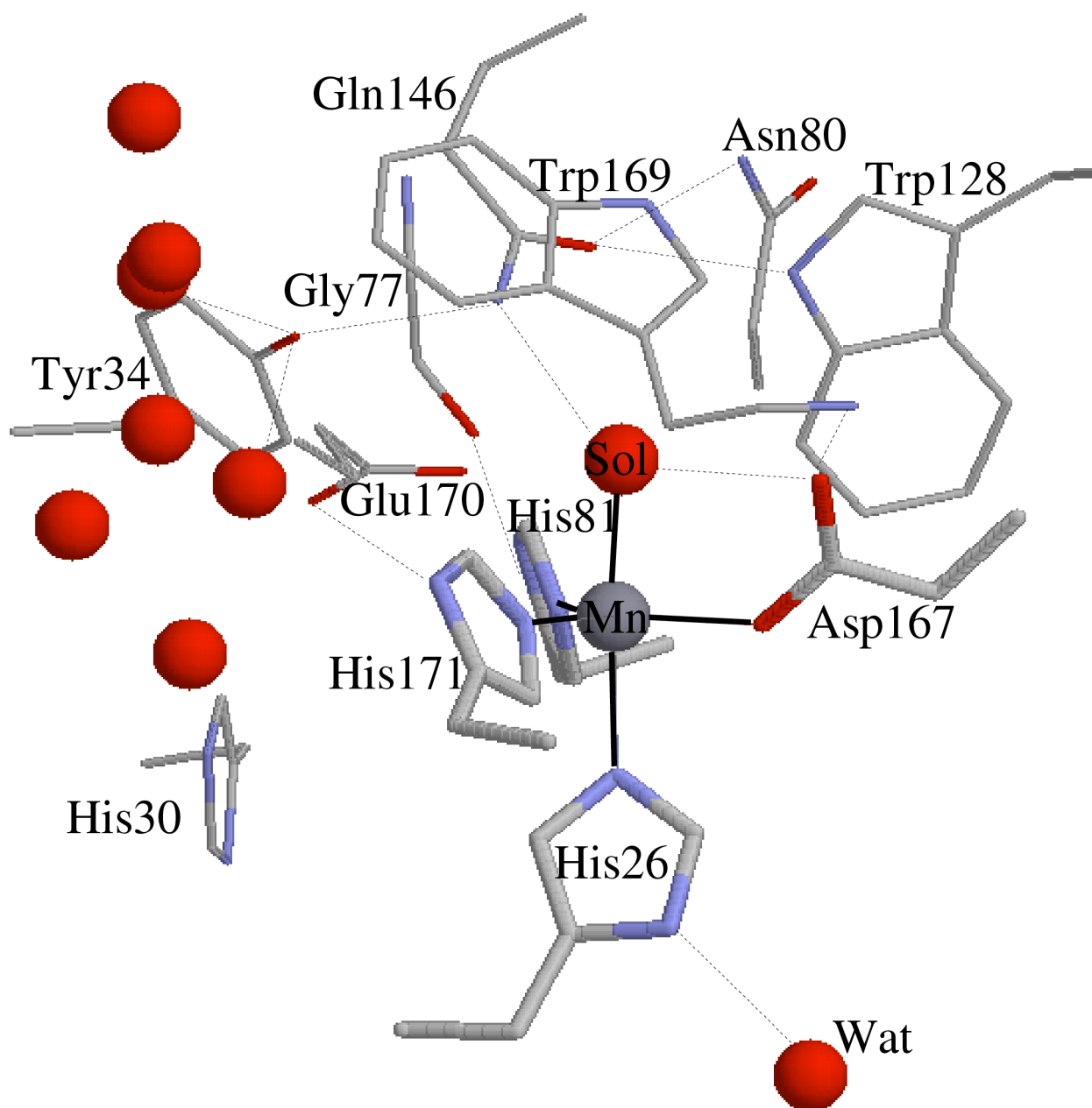
Figure 3. Residues and hydrogen bonds around the active site in the crystal structure of MnSOD. 16 Mn ligands are shown in thick coloured lines, other ligands in thinner lines, and water molecules as red balls. Coordinative bonds are shown in thick black lines, hydrogen bonds in thin, dotted lines.
