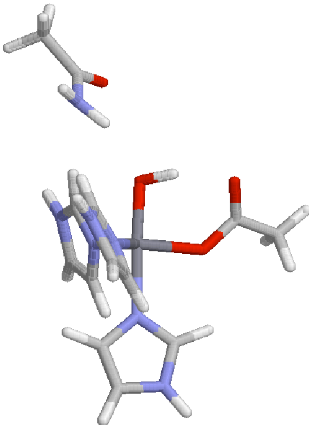
Figure 1. The quantum system used in the calculations (illustrated by the \text{Mn}^{3+}\text{Im}_3\text{AcOH}+\text{Am} model).
