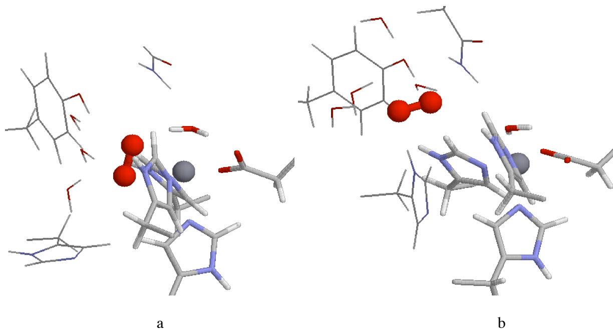
Figure 5. The two binding modes of O_2^{\bullet-} to MnSOD observed in the molecular dynamics simulations. The metal ion and the O_2^{\bullet-} molecule are shown as balls, the Mn ligands, as thick stick, whereas His-30, Tyr-34, Gln-147, as well as a few nearby water molecules are shown as thin sticks.
