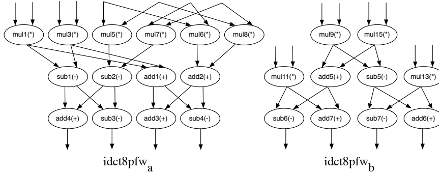
Figure 1: idct8pfw Slepniir instruction that covers the half of Loeffler’s IDCT algorithm [18]
