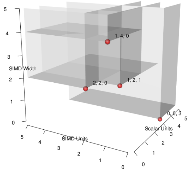
Figure 3: The Pareto points obtained for IDCT.
