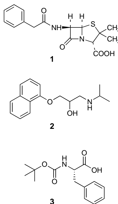
Scheme 1. Structure of Penicillin G ( 1 ), Propranolol ( 2 ), and Boc-L-Phe-OH ( 3 ).
