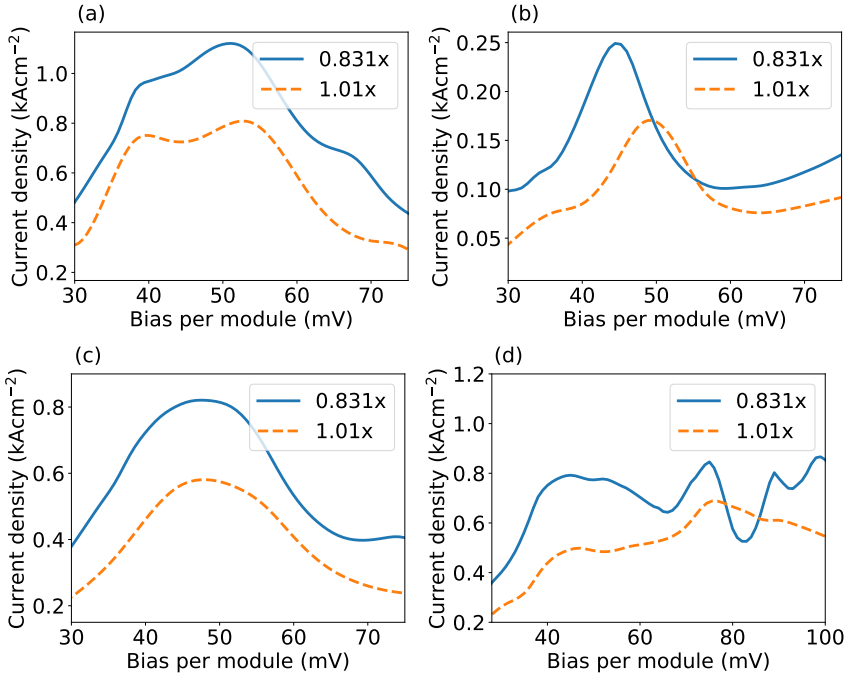
Figure 5.2: Current and bias relation without lasing is shown for four structures discussed in Fig. 5.1. Full lines are calculated with 0.831x eV and dashed lines are with 1.01x eV conduction band offsets. The devices studied here are ChassagneuxIEEE2012, KumarAPL2006, WilliamsElecLett2004 and KumarNature2010 for (a), (b), (c) and (d) respectively. Phonon temperatures are fixed in each panel at 150 K.
