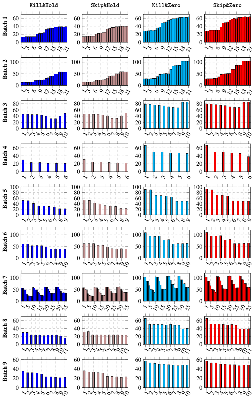
Figure 6. Performance Recovery Interval n_{H}^* needed to recover from a burst of 10 deadline misses for different strategies and all the plants in the 9 batches for PI controllers designed according to [Garpinger and Hägglund, 2015].
