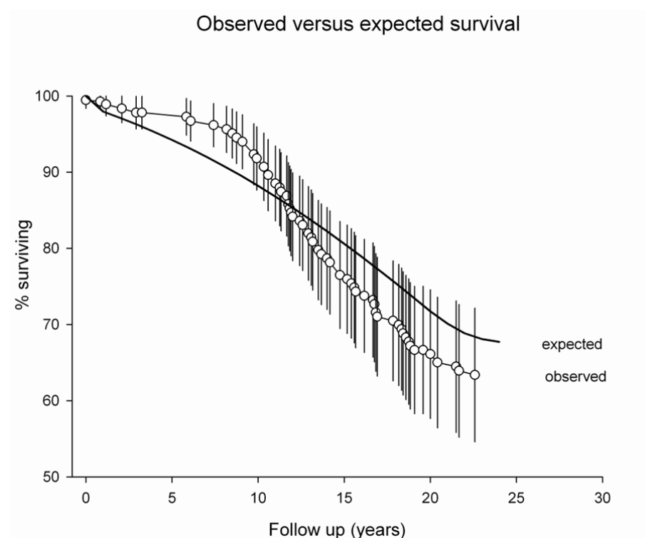
Figure 1. Long-term survival (95% CI) among patients with RA followed prospectively since disease onset. Comparison with survival expected in Sweden for the same time period, adjusted for calendar year, age, and sex.
