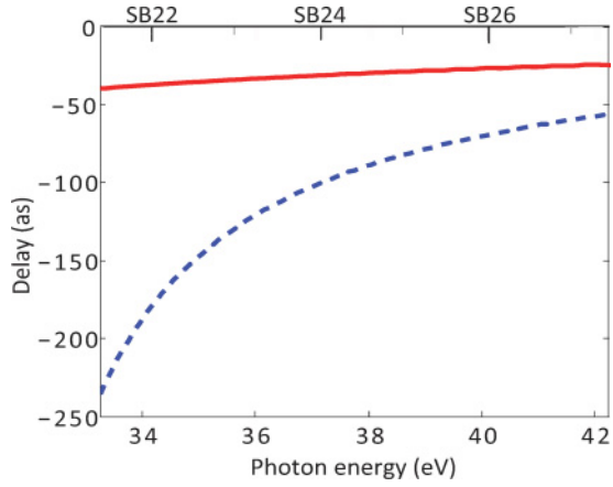
FIG. 5. (Color online) Continuum-continuum delay \tau_{cc} as a function of excitation photon energy for subshells 3s (red solid line) and 3p (blue dashed line) for an IR photon energy of 1.55 eV ( 800 -nm wavelength).
