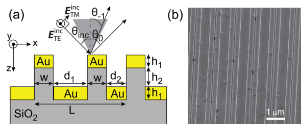
FIG. 1. (Color online) (a) Schematic of a DLG of period L . The (long) axes of the Au wires are parallel to the y direction. The direction of the incident light lies in the xz plane and is defined by \theta_{inc} . As examples, the directions of the 0th and -1st diffracted orders are specified and marked by \theta_0 and \theta_{-1} in the figure. The shaded triangle indicates the cone of the light collected by an objective lens with NA = 0.5 oriented normal to the DLG. E_{TE}^{inc} \parallel e_y and E_{TM}^{inc} \perp e_y define the TE and TM polarized components of the electric field of the incident light. (b) SEM image (the top view) of a fabricated DLG with d_1 = 500 nm, d_2 = 100 nm, w = 200 nm, h_1 = 60 nm, and h_2 = 30 nm. The scale bar is 1 \mu m.
